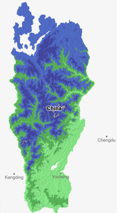
Figure 4.6. Future Climate Classifications
