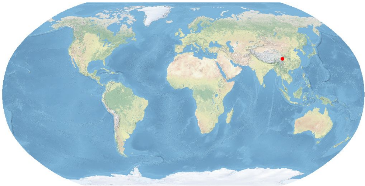
Location of the Qionglai Shan mountain range [1][2].
