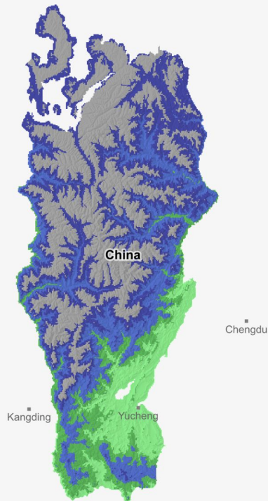
Figure 4.5. Current Climate Classifications
