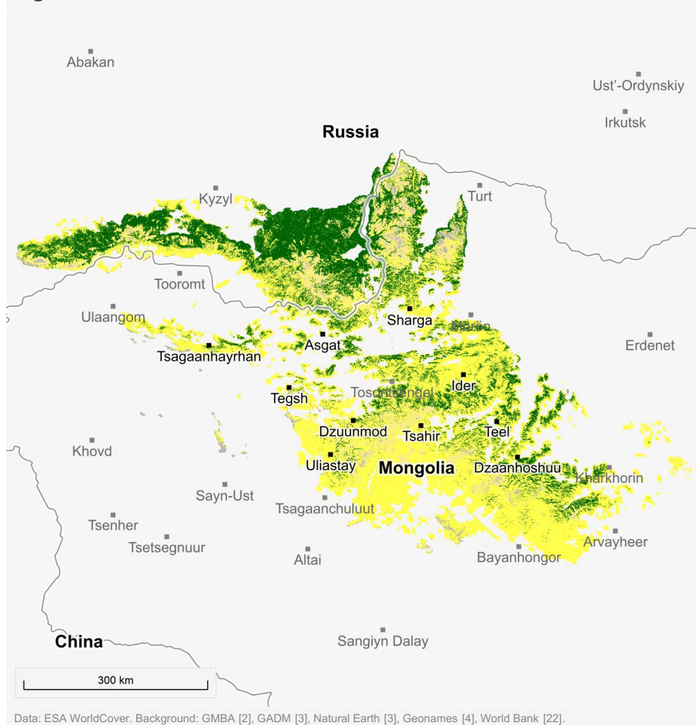
Figure 2.1. Land Cover
