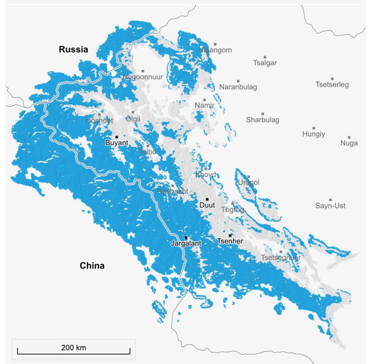
Figure 6.4. Mean Snow Covered Area (January)
