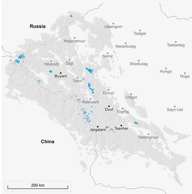
Figure 6.3. Mean Snow Covered Area (July)
