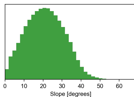
Figure 3.3. Distribution of slope steepness within in the mountain range [21].
