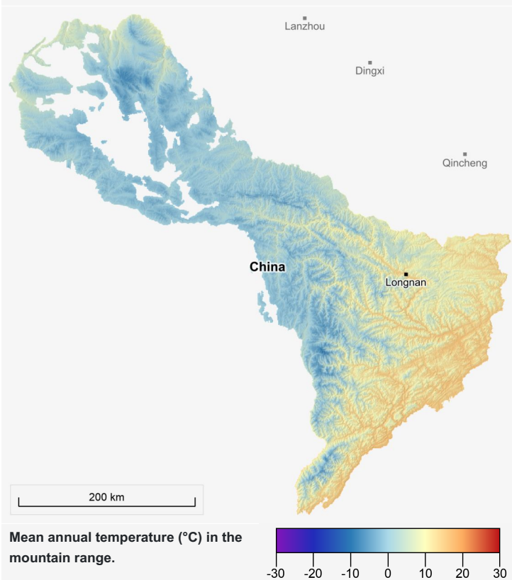
Figure 4.1. Mean Annual Temperature
