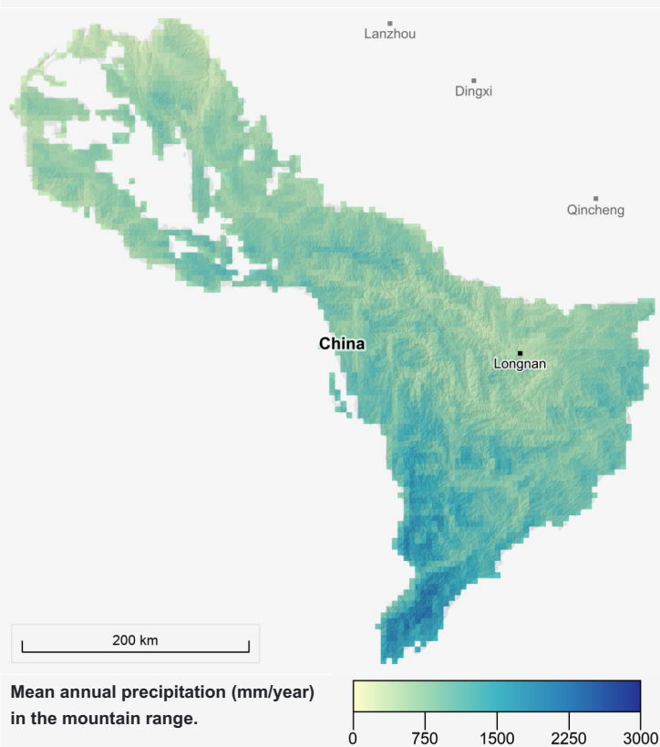
Figure 4.2. Mean Annual Precipitation
