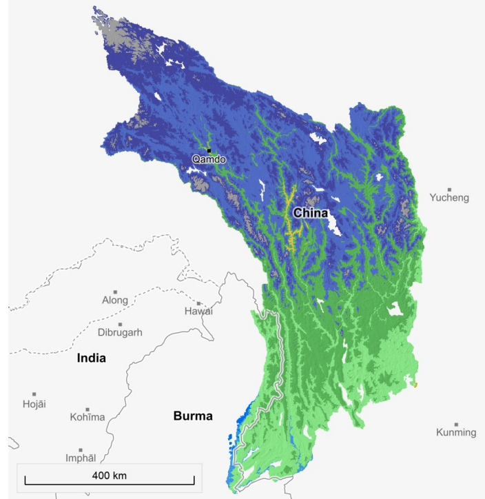
Figure 4.6. Future Climate Classifications
