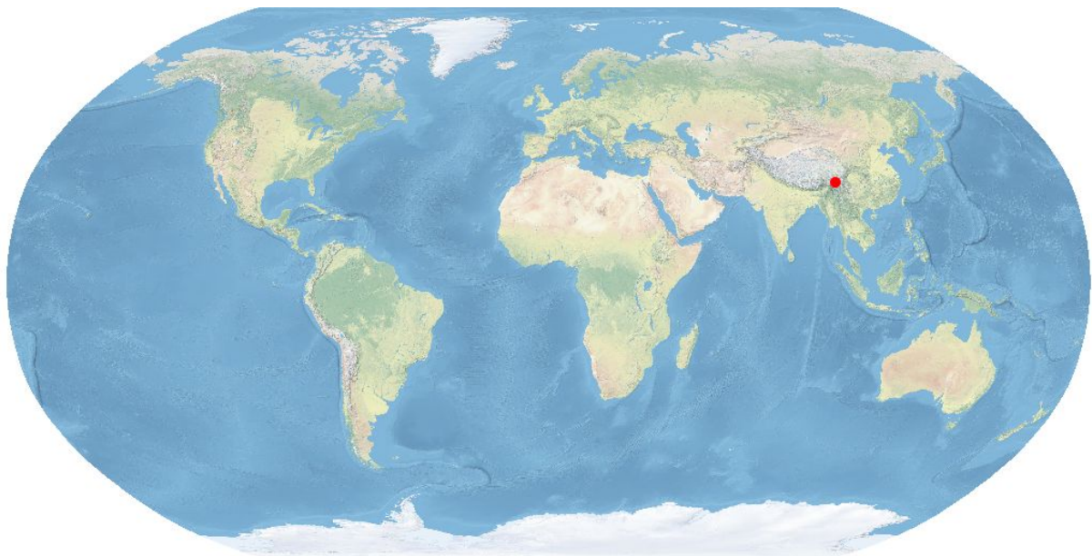
Location of the Hengduan Shan mountain range [1][2].
