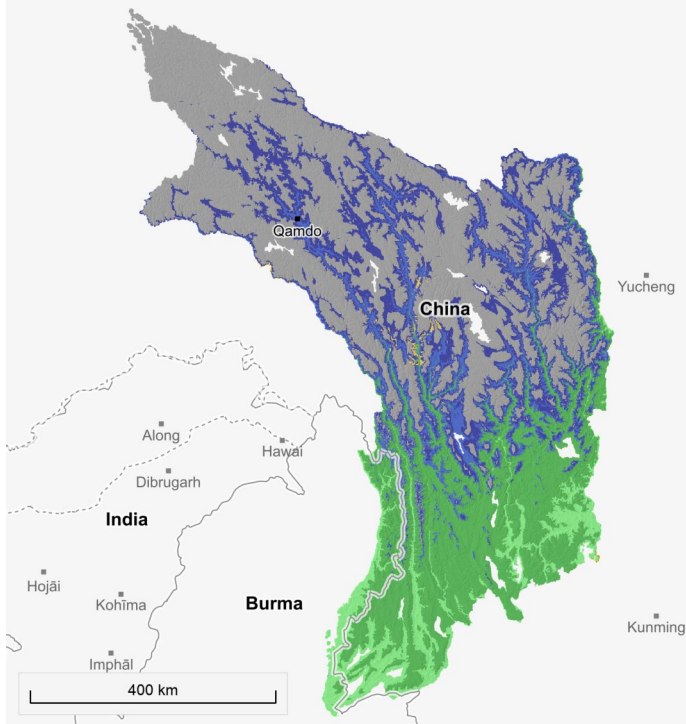
Figure 4.5. Current Climate Classifications
