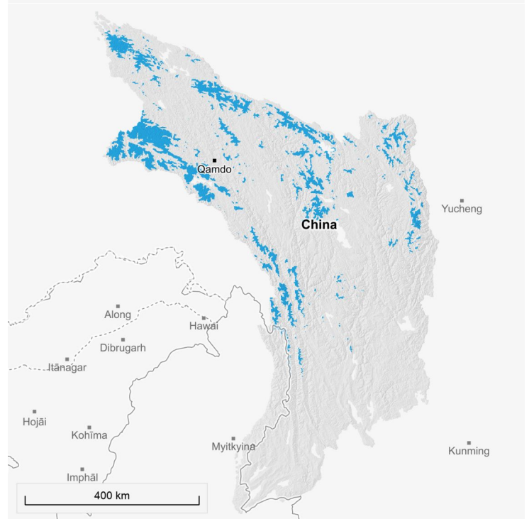
Figure 6.4. Mean Snow Covered Area (March)
