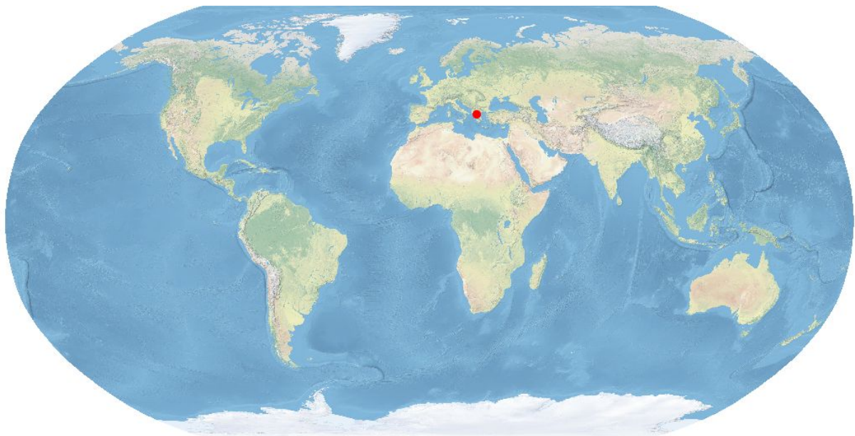
Location of the Hellenides mountain range [1][2].
