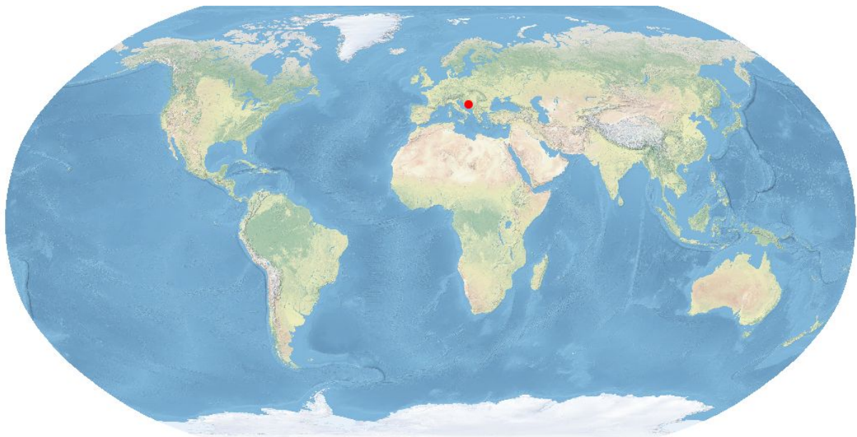
Location of the Dinaric Alps mountain range [1][2].
