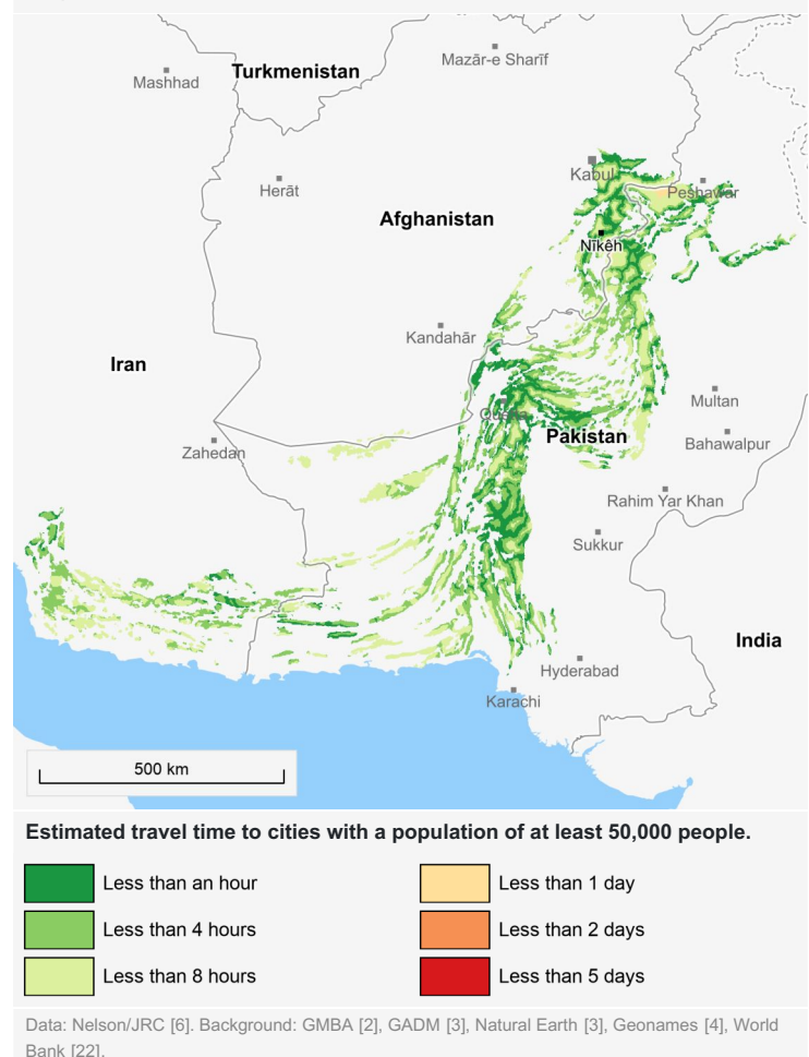
Figure 1.4. Travel Time
