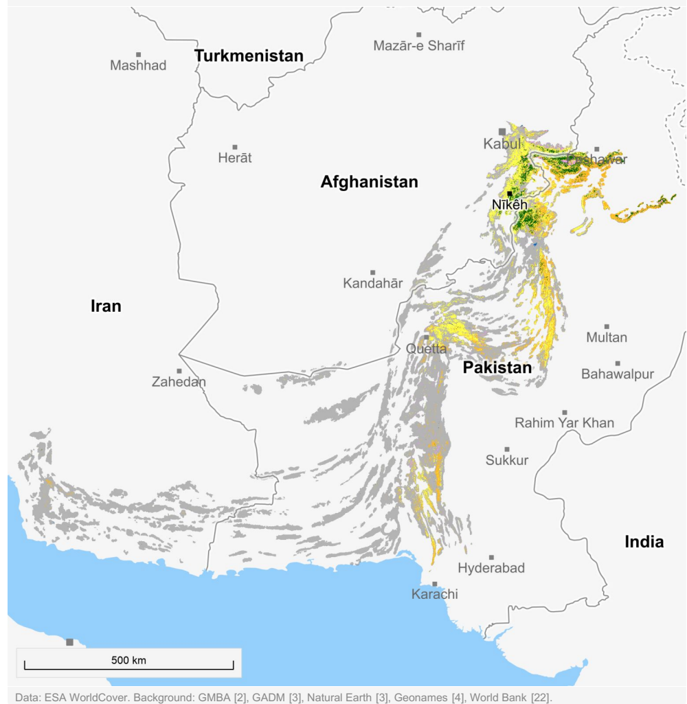
Figure 2.1. Land Cover
