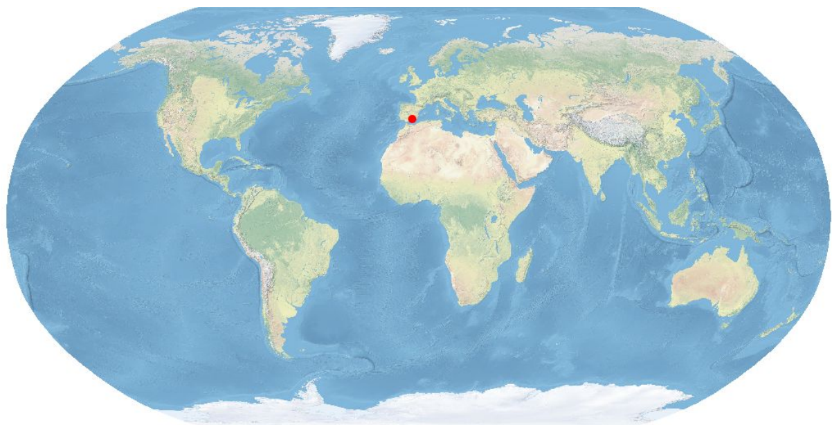
Location of the Baetic System mountain range [1][2].
