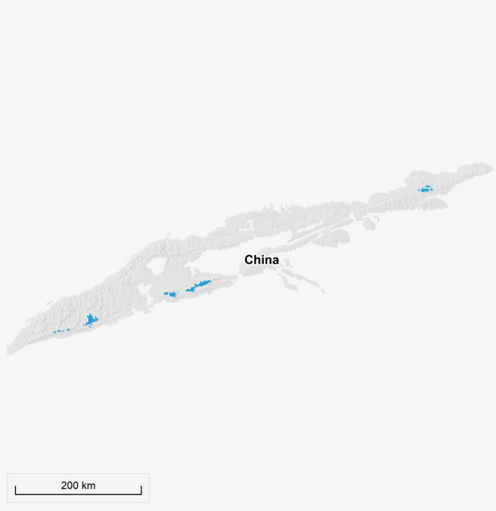
Figure 6.3. Mean Snow Covered Area (August)
