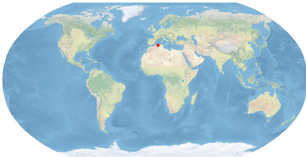
Location of the Tell Atlas mountain range [1][2].
