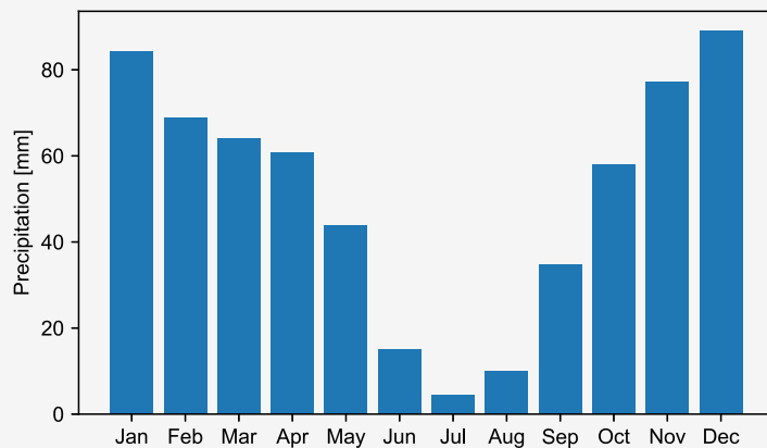
Figure 4.4. Mean Monthly Precipitation
