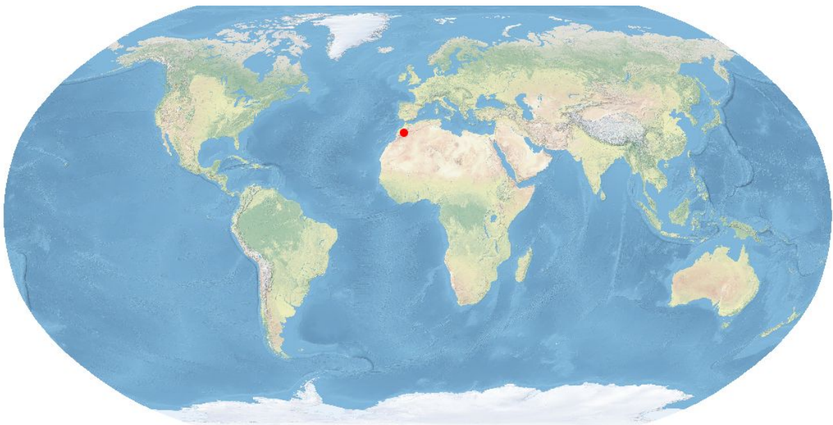
Location of the High Atlas Range mountain range [1][2].
