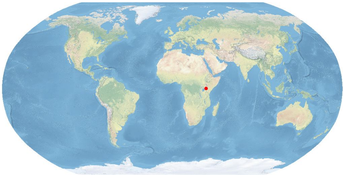
Location of the Eastern Rift mountains mountain range [1][2].
