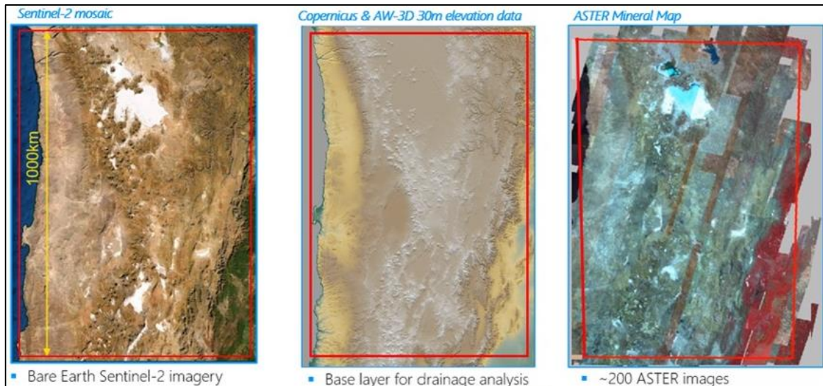
Figure 1. The use of optical Sentinel-2 imagery for the geological mapping, Copernicus and AW3D elevation data for the drainage analysis and ASTER for multi-spectral clay alteration mapping have enabled large-footprint paleosalars to be outlined.
