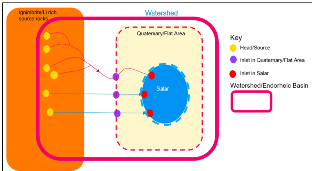
Figure 2. A model detailing the key attributes in the lithium-brine mineral system and how it equates to a Source-to-Sink model.
