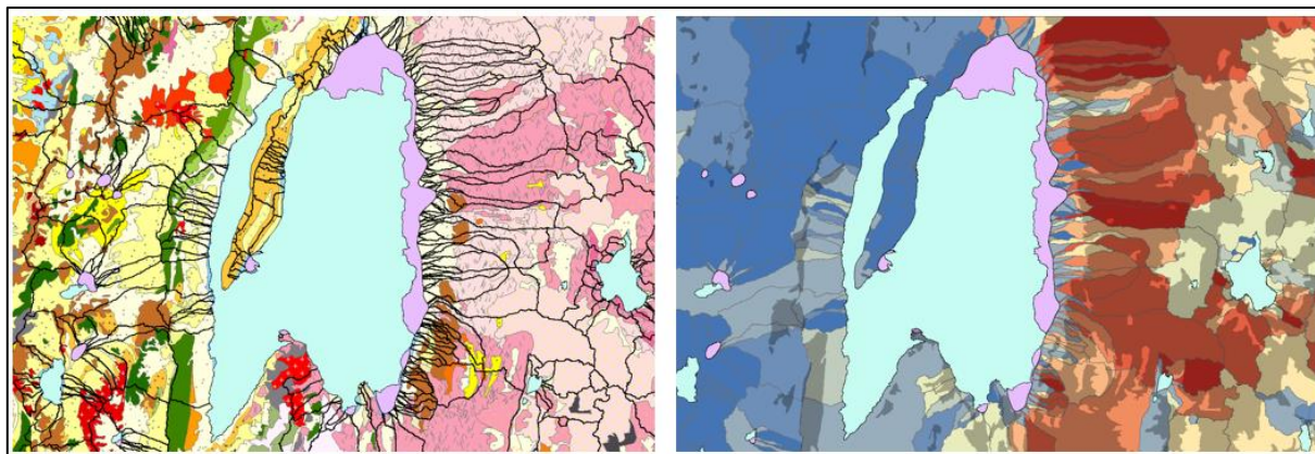
Figure 3. Salar de Atacama is shown in the sky-blue in the centre (~50 km wide). The left-hand image has the geological interpretation and the watershed areas of the rivers within the endorheic basin (black polygons). The lilac area to the east of the salar is a Quaternary flat area as outlined by the elevation data. To the right the ranked lithium-rich source rocks (shades of red) have numerous inlets into this flat area and therefore make it of interest for exploration.
