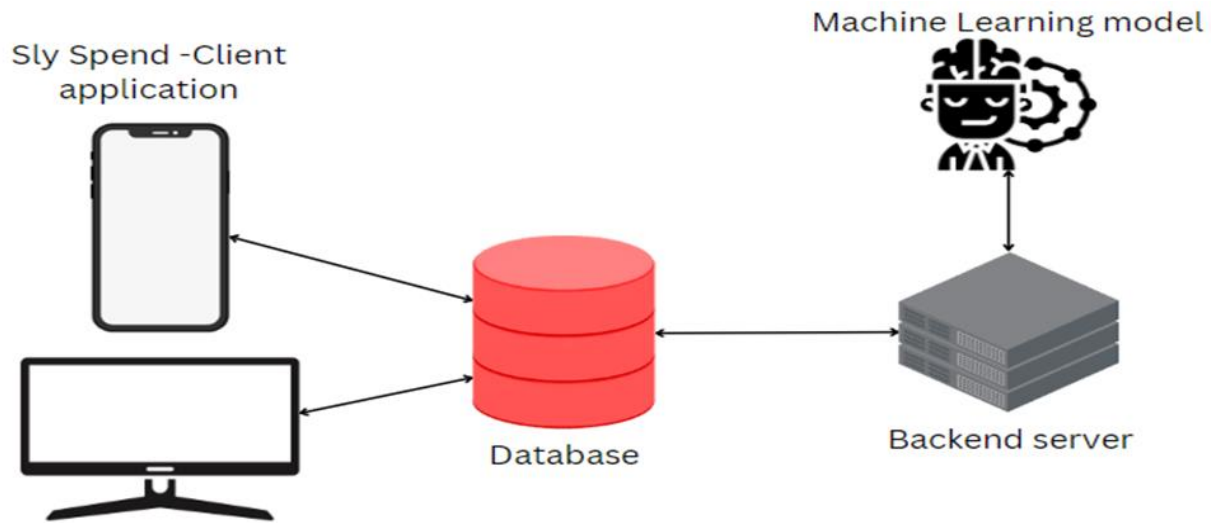
Fig. 4 Architecture Mode
