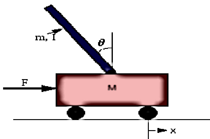
Figure(3): Free body diagram of the Inverted Pendulum
