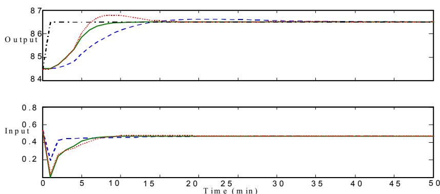
Figure(2): Closed-loop response for non-linear system with PID controller parameters based on relay feedback (dotted line), a plant step response based technique (dashed line) and NCD (solid line).
