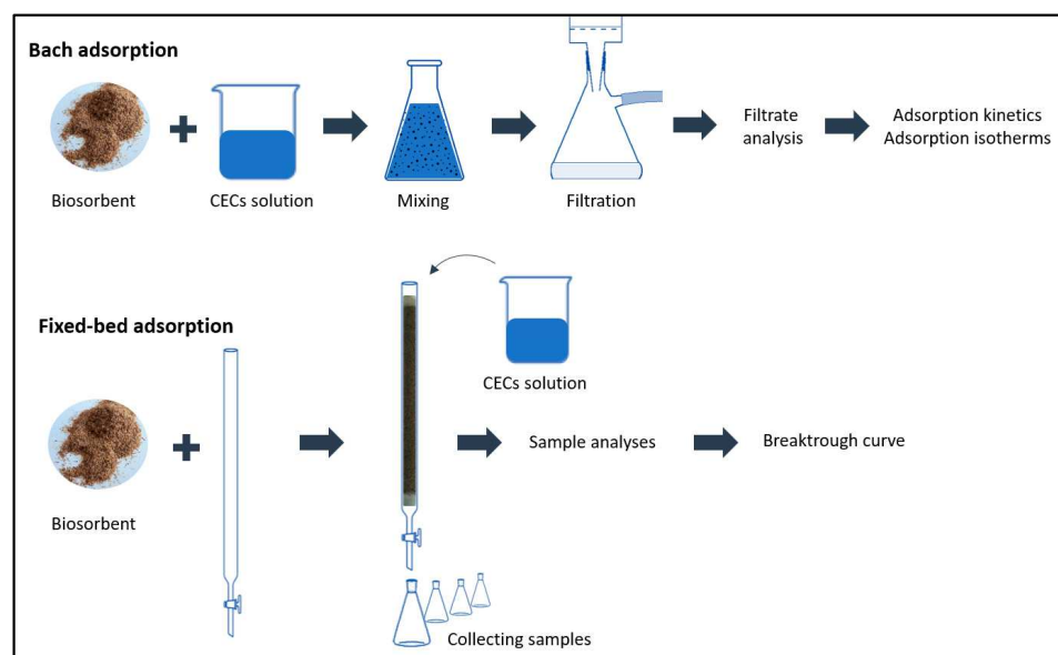
Figure 1. Schematic representation of batch and continuous adsorption methods.
