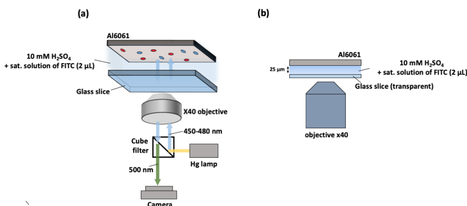
Fig. S1-1 Schemes (not to scale) (a) of the entire setup for an operando fluorescence microscopy observation of the mirror polished Al6061 interface exposed to 10 mM H 2 SO 4 + sat. FITC solution and (b) of the solution cell.
