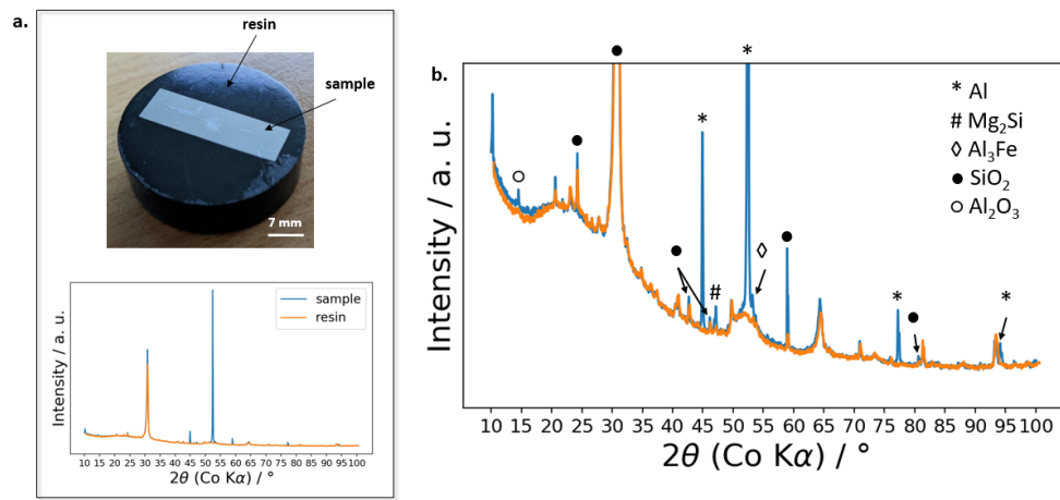
Fig. S5-1 (a) Macroscopic picture of Al6061 sample placed into the resin (top) and the diffractograms of individual resin and sample embedded into resin (bottom). (b) Zoomed diffractogram with peak attribution: Al (ref ICSD 98-004-3492), Mg 2 Si (ref ICSD 98-016-7510), Al 3 Fe (ref. [18]), SiO 2 (ref ICSD 98-015-6198) and Al 2 O 3 (ref ICSD 98-017-3014). Ensemble of small peak, related to resin, are not marked but attributed to graphite (ref ICSD 98-007-6767).
