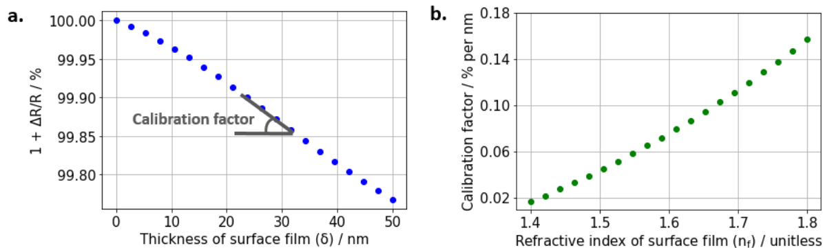
Fig. S1-3 (a) Calculated change in reflectivity as a function of the surface film thickness using eq. 2 for Al/Al(OH) 3 /H 2 O interface at \lambda = 490 nm, n_S^{Al} = 0.46 + 4.69i , [7] n_F^{Al(OH)_3} = 1.67 [8] and n_A^{H_2O} = 1.33 . [7,8] (b) shows the sensitivity (ratio between reflectivity change in % per nm of surface film) as a function of the refractive index of surface film n_f .
