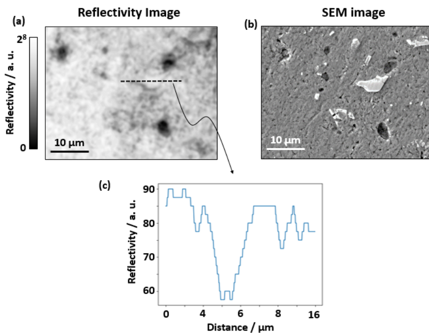
Fig. S6-1 (a) Reflectivity and (b) SEM image of identical locations taken from Fig. 1b from the main manuscript. (c) presents the 2D profile of intensity of reflected light along the dash line in figure (a).
