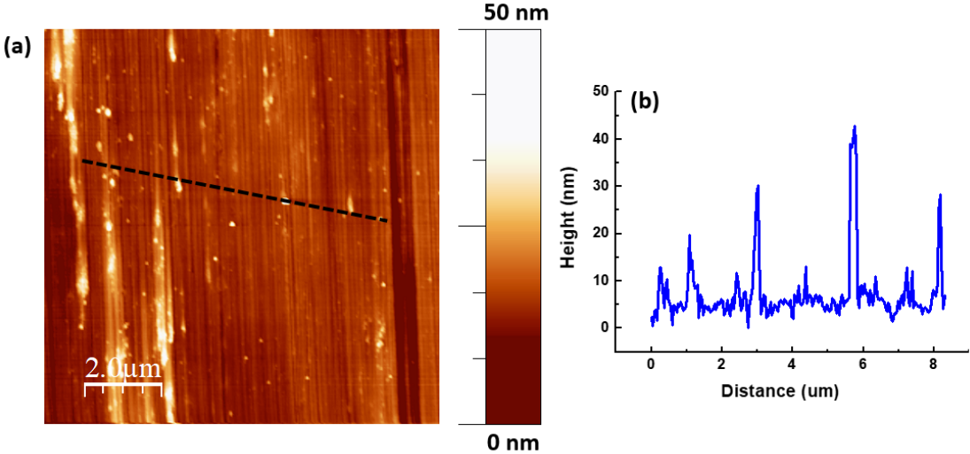
Fig. S3-1 (a) Typical AFM image of mirror polished Al6061 samples and (b) is the 2D section along the back dash line in (a)
