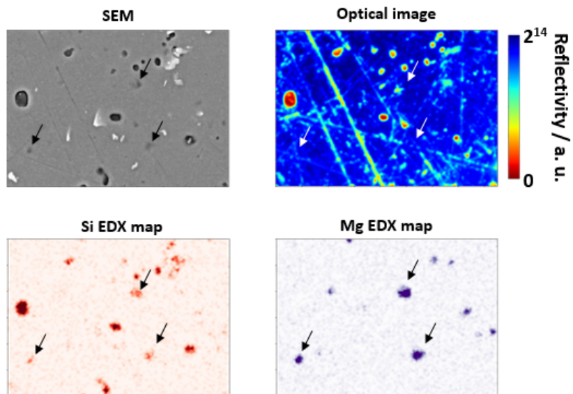
Fig. S4-2 Zoom of the maps in Fig. S4-1 showing SEM, Si and Mg EDX maps complemented with optical image. Identical locations that correspond to the most intense Mg spots on EDX map are highlighted with arrows in all four images.
