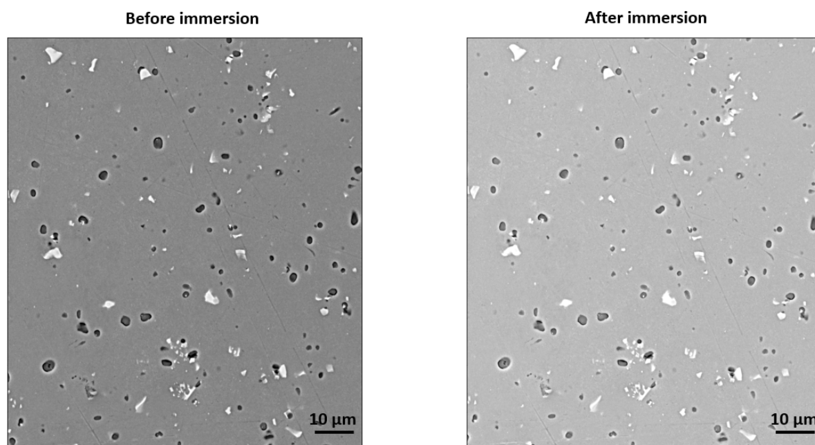
Fig. S4-1a Representative SEM images of Al6061 surface before and after 5 min immersion in 10 mM H_2SO_4 aqueous solution. Slightly different contrast between images is due to contrast differences set in SEM image acquisition software and is not related to the differences in the surface states. Below we provide EDX maps of Si, O, Fe and Mg distribution.
