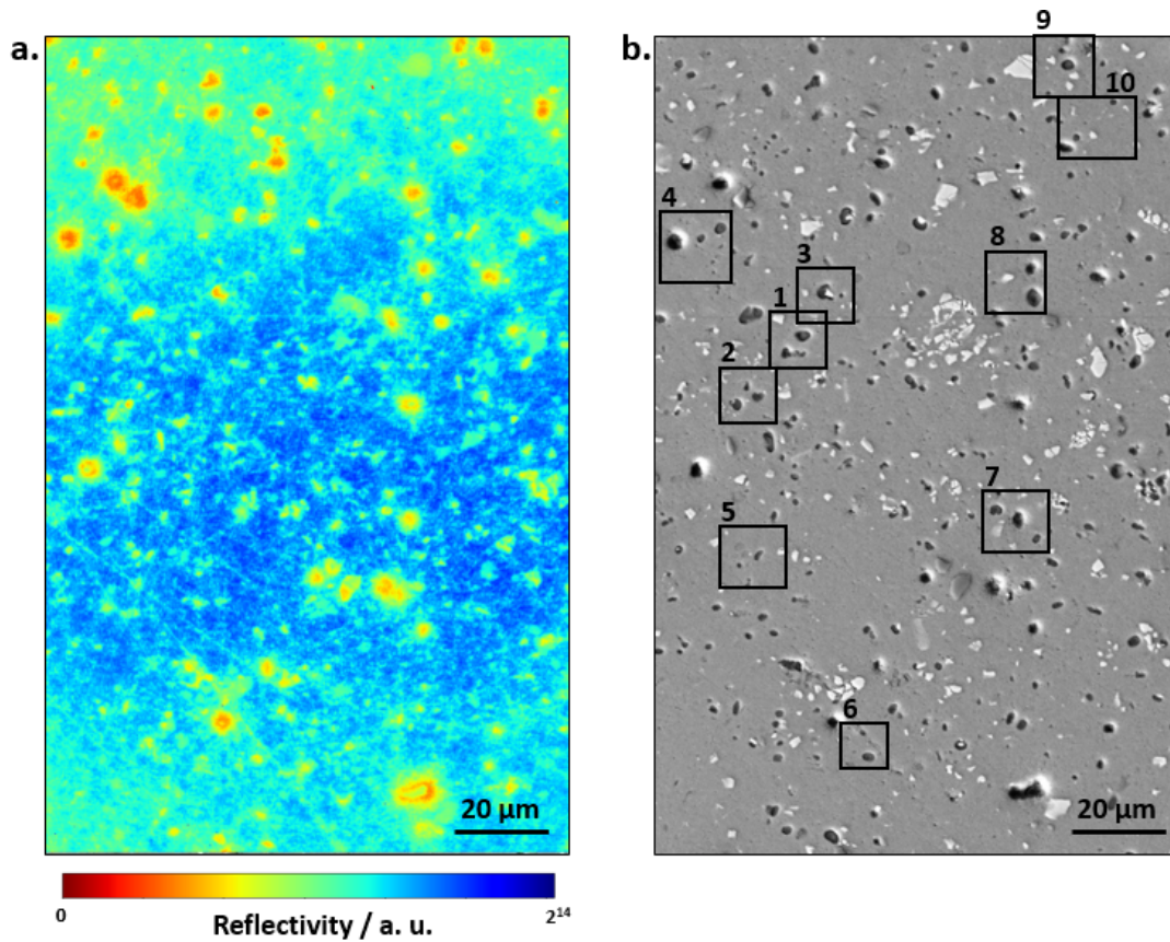
Fig. S7-1 (a) Wide-field optical and (b) SEM images of analyzed Al6061 interface. Regions, where the crosstalk was suspected, are highlighted with rectangles.
