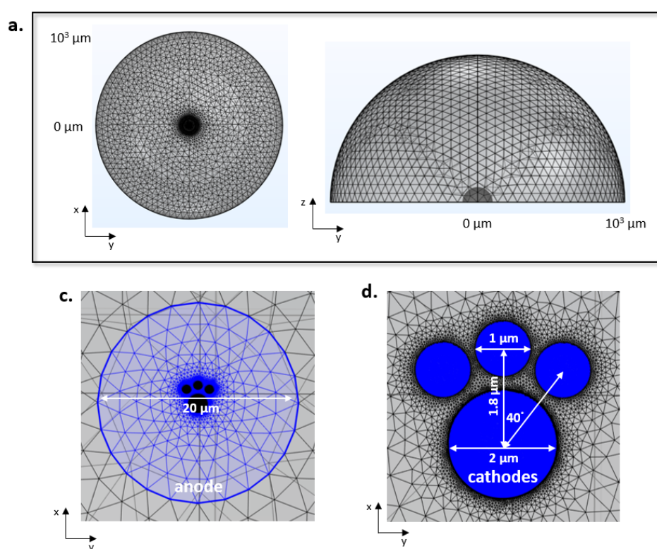
Fig. S2-1 Geometry (up to scale) of the simulated box in FEM model. (a) show the whole view in xy and zy planes while (c) is the zoom of the whole electroactive area located at the bottom of simulated hemisphere (the anode area is highlighted with blue) and (d) is the zoom around 2D disks, where the cathode areas are highlighted in blue. Triangles represent free tetrahedral meshing employed in the model.
