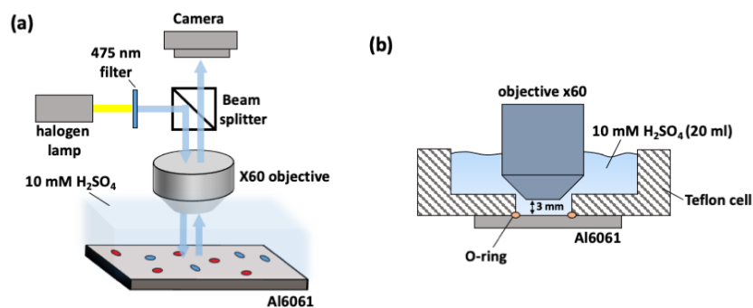
Fig. S1-2 Schemes (not to scale) (a) of the entire setup for an in-situ reflective microscopy observation exposed to 10 mM H 2 SO 4 and (b) of the solution cell.
