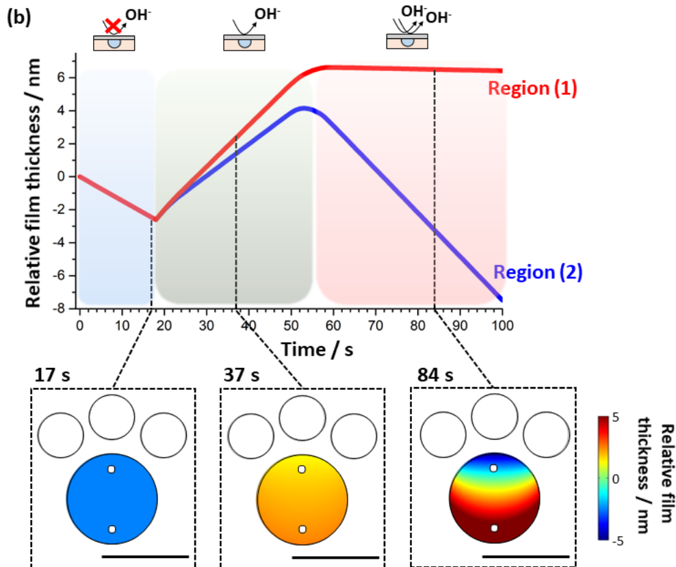
1 2 Fig. 3 Overview of FEM simulations. (a) Left, size and position of the cathodic and anodic 3 regions with a brief summary of electrochemical reactions considered. Right, steady-state pH 4 distribution over cathodic zones, showing the pH gradient over the largest cathodic region. 5 Regions 1 and 2 are highlighted in analogy to those chosen from the experimental observations 6 in Fig. 2. (b) Top, evolution of relative film thickness in regions 1 and 2. The schemes on top of 7 the film thickness evolution depict the activity of the cathodic particles in each regime. Bottom, 8 the spatial distribution of the relative film thickness over the large cathodic region after 17, 37 9 and 84 s of simulations. The scale bars are 2 \mu\text{m} .
