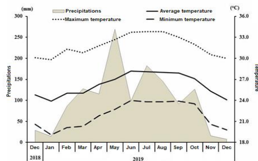
Fig. 1. Monthly means of temperature and precipitation throughout the research.
