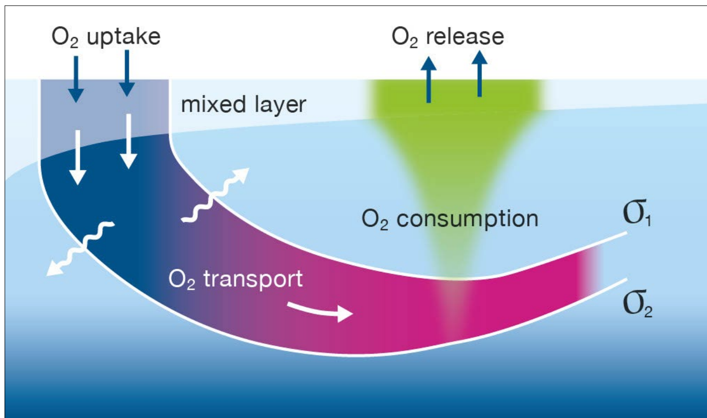
Figure 3.4 Schematic representation of oxygen uptake and release, physical transport, and biological production and consumption in the Ocean. Oxygen is mostly taken up into the Ocean in the cold waters of the high latitudes, in which oxygen is most soluble. When this water sinks into deeper waters, it oxygenates deeper parts of the Ocean. Transport of oxygen in the interior of the Ocean happens along density layers (isopycnals marked as \sigma_1 and \sigma_2 ). Some organic matter (green) produced by photosynthesis in the surface Ocean sinks and oxygen is consumed through its respiration throughout the water column, leading to a decline in oxygen as water flows from the poles to the equator in the Ocean's interior (the colour change from blue to pink illustrates the decreasing oxygen concentration from oxygen-rich waters originating in the poles).
