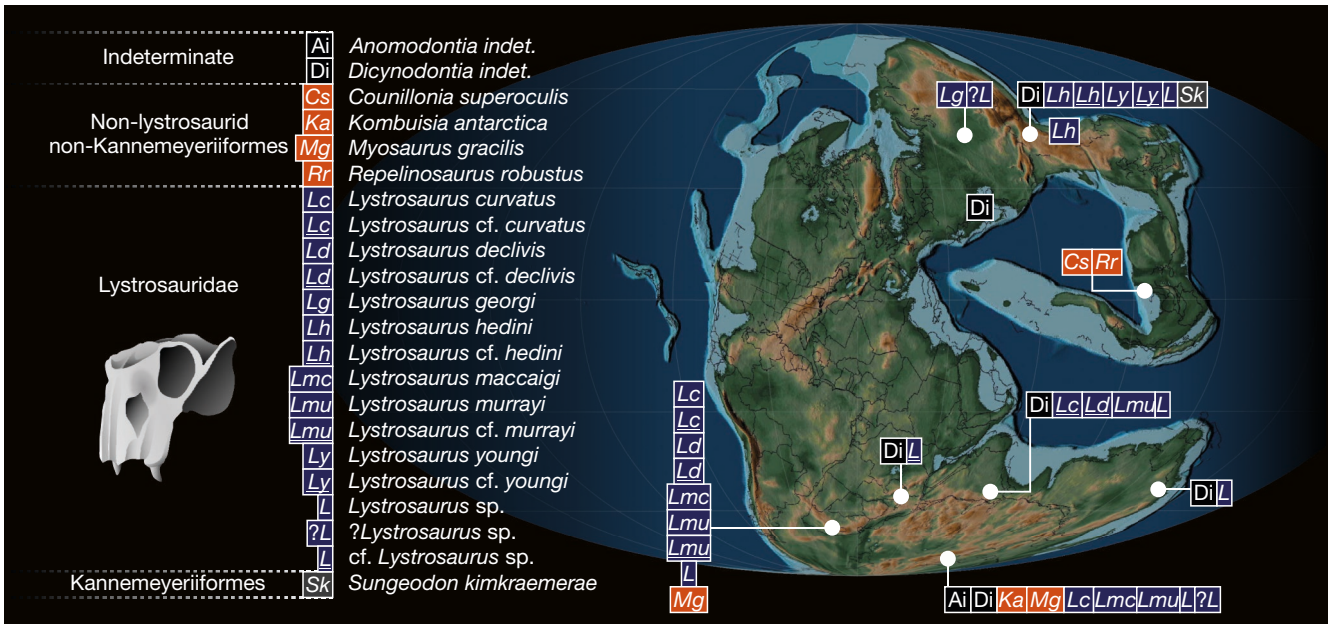
FIG. 20. — Early Triassic distribution of dicynodont finds. Skull of Lystrosaurus declivis (Owen, 1859) based on UCM 42870.
