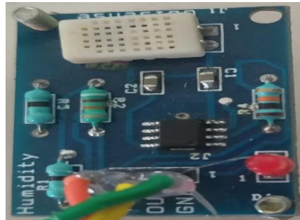
Figure.4. Humidity Sensor
