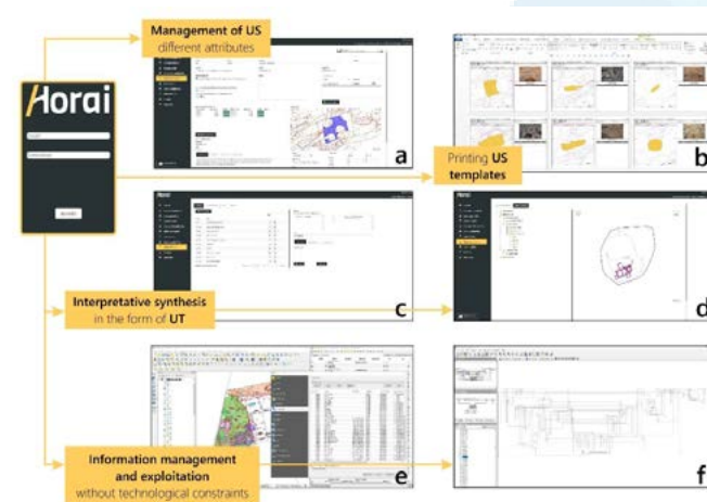
Figure 1. HORAI interface and some platform's functionalities. Amongst these, there are those dedicated to US description themselves (a) along with their automated printing templates (b); the US clustering captured as UT (c, d, f); and examples for management and exploitation on other interconnected software (e, f).
