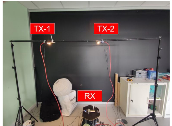
Fig. 3. Experiment setup for hybrid VLC/WiFi testbed
