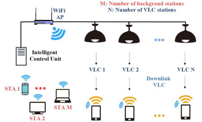
Fig. 1. Simple scenarios for hybrid VLC/WiFi network
