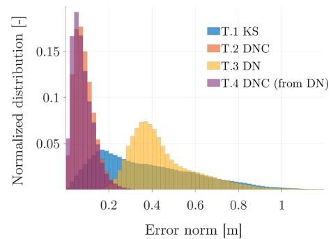
Fig. 9. Normalized distribution of point cloud georeferencing error in magnitude for the four trajectories.
