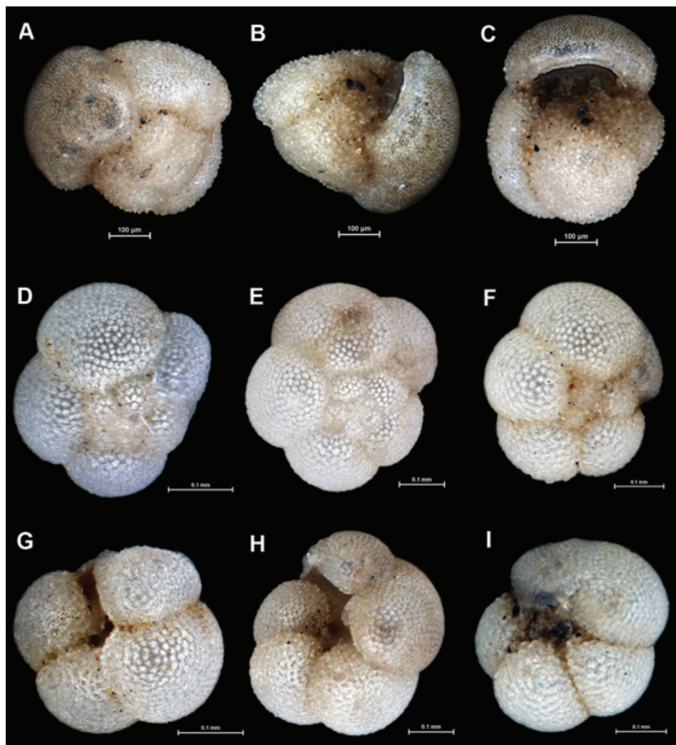
Fig. 4. (A–C) Globorotalia inflata (d’Orbigny, 1839), sample 26; (D, G) Neogloboquadrina incompta , sample 15; (E, H) N. dutertrei (d’Orbigny, 1839), sample 30; (F, I) N. dutertrei , a low trochospiral specimen with more umbilical aperture from sample 30.
