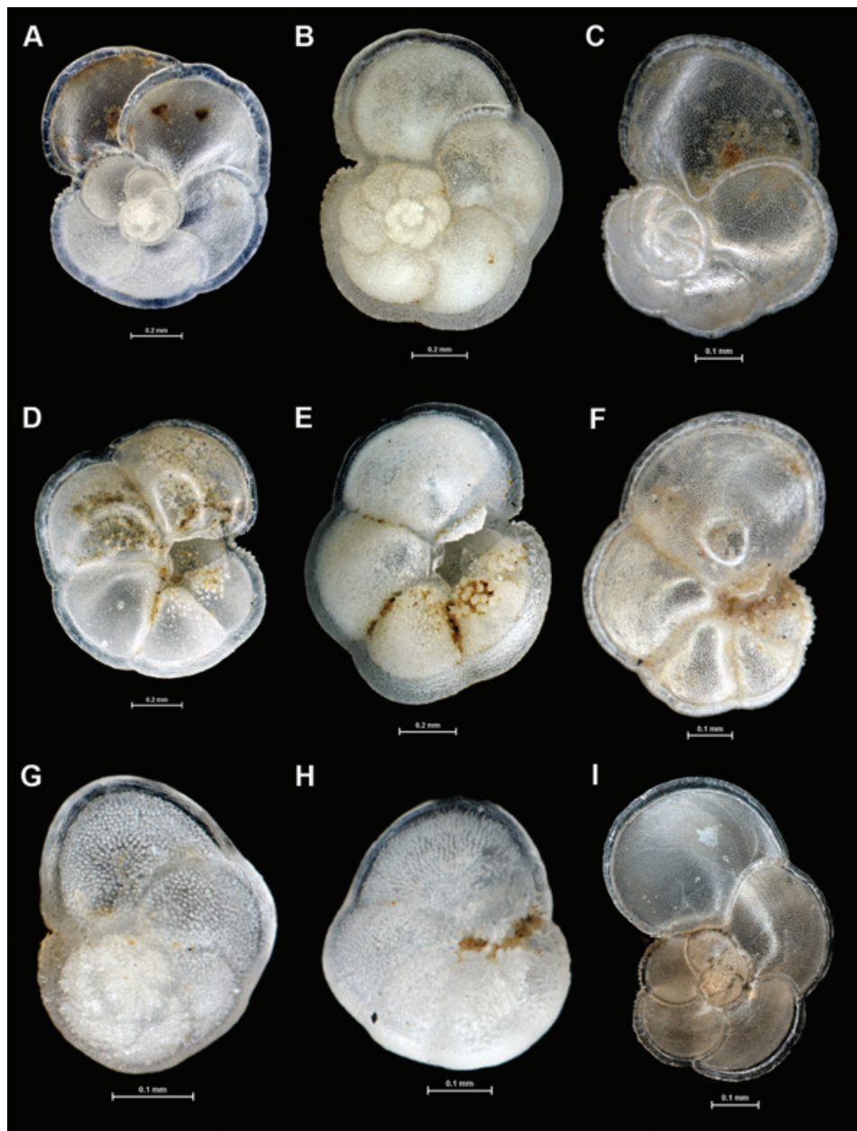
Fig. 3. (A, D) Globorotalia cultrata (d'Orbigny, 1839), sample 25; (B, E) Globorotalia menardii (Parker, Jones & Brady, 1865), sample 30; (C, F) Globorotalia ungulata Bermúdez, 1961, sample 25; (G, H) Globorotalia tumida (Brady, 1877), sample 26; (I) Globorotalia ungulata Bermúdez, 1961, sample 30.
