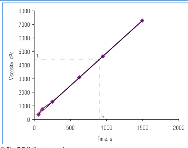
Fig. 3.5 Calibration graph
