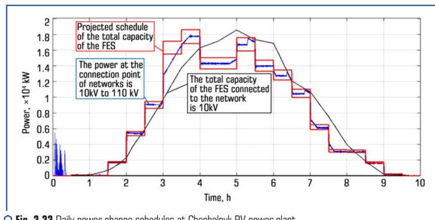
○ Fig. 2.22 Daily power change schedules at Chechelnyk PV power plant
