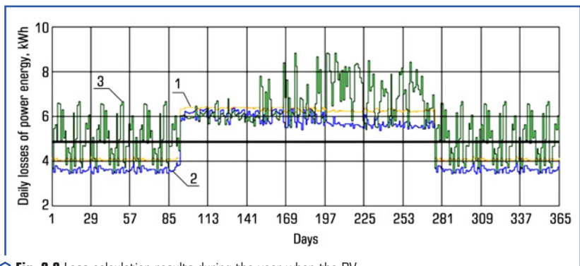
○ Fig. 2.2 Loss calculation results during the year when the PV power plant is installed at node 20
