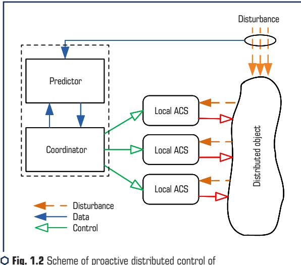
Fig. 1.2 Scheme of proactive distributed control of a distributed object
