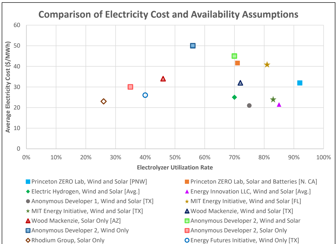
Figure 2: Average electricity cost and electrolyzer utilization rates from each study that reported these metrics, including multiple cases where available. Filled markers indicate studies that allowed both oversizing of clean generating capacity and sales of excess clean generation. Patterned markers indicate studies that allowed oversizing but not excess sales. Unfilled markers indicate studies that assumed clean generating capacity to be equal to electrolyzer capacity.
