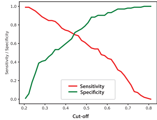
k-NN chebyshev
