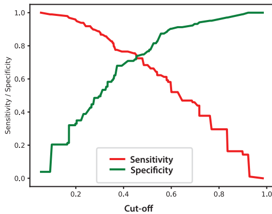
LR - liblinear
