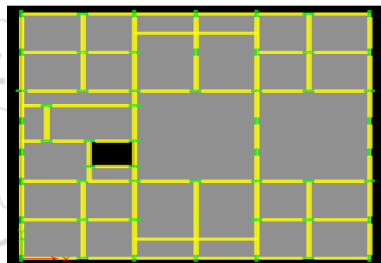
Figure 3.2: Structural layout for regular shape
