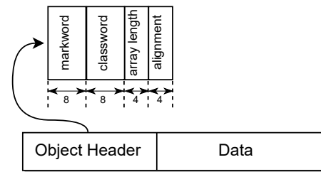
Figure 2: The layout of an object that stores an array in JVM when CompressedOops are disabled.
