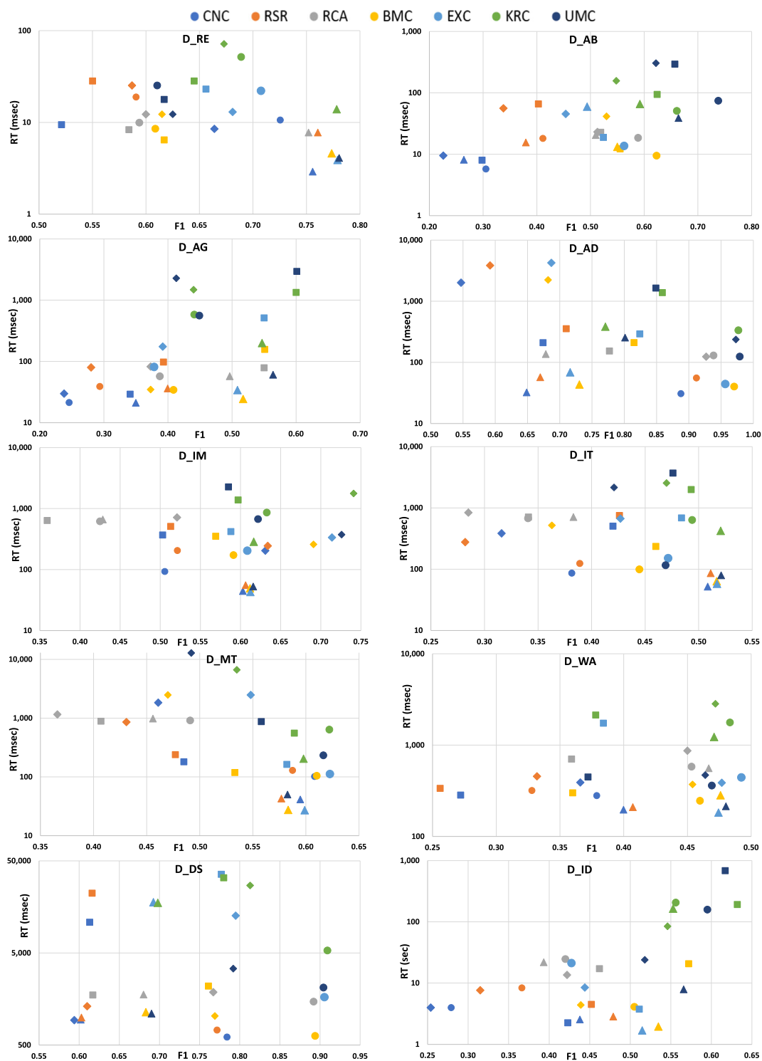
Fig. 12 Scatter plots of the average F1 (on the horizontal axis) and the average run-time (on the vertical axis) per algorithm and type of edge weights across all data sets. Every algorithm corresponds to a different color, as explained in the legend, and every type of input to a different color shape: circle stands for the schema-agnostic syntactic weights, triangle
