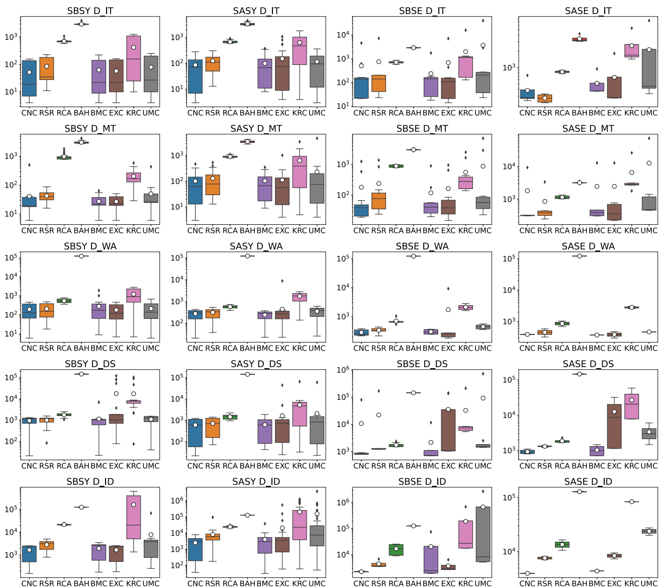
Fig. 8 The distribution of run-time (in ms) per algorithm and type of edge weights across the five largest data sets. Every row corresponds to a different data set. Note the log-scale of the vertical
