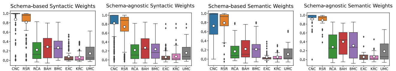
Fig. 15 The deviation in F1 between the fine-tuned threshold and the automatically configured one, i.e., Mean + SD, across all algorithms and types of edge weights
