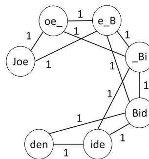
Fig. 3 The 3-gram graph corresponding to the string value “Joe Biden”
