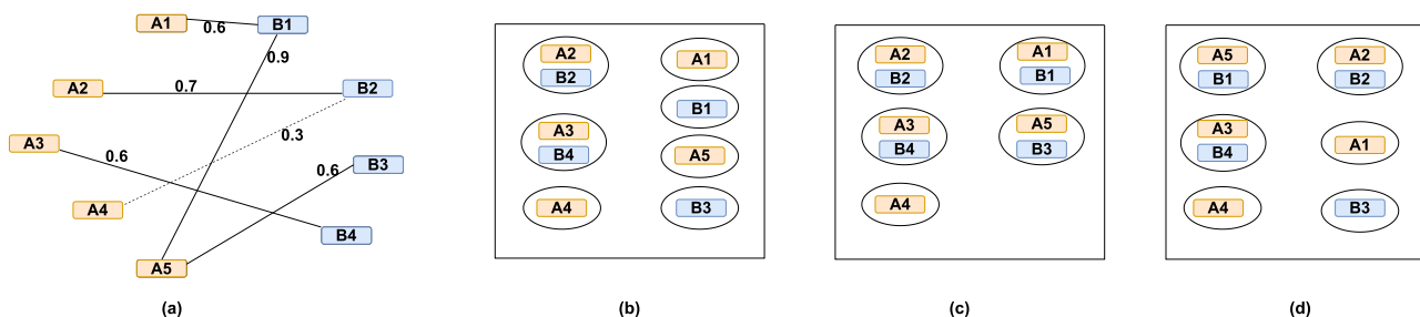
Fig. 1 Example of processing a bipartite similarity graph with a similarity threshold of 0.5 (i.e., edges with a lower score such as A4–B2 are ignored): a the similarity graph constructed for a pair of clean data sets ( V_1 in orange and V_2 in blue), b the resulting clusters after applying CNC, c the resulting clusters assuming that the approximation algorithms RCA
