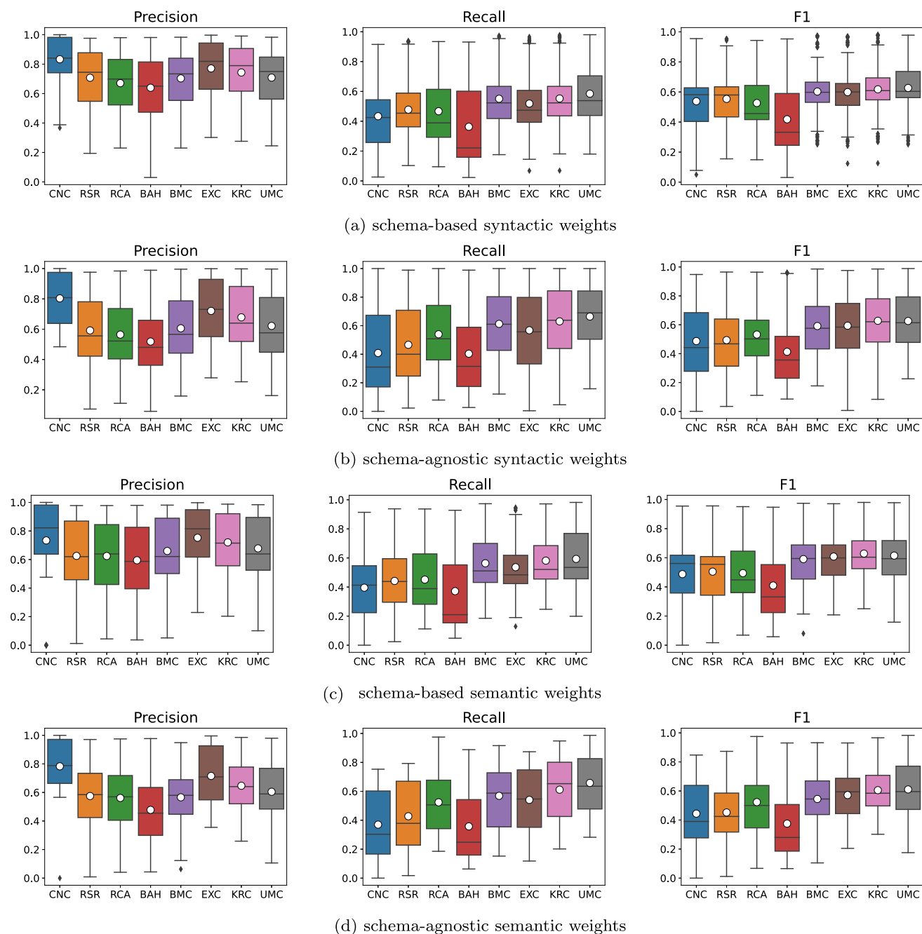
Fig. 6 Precision, recall and F1 of all algorithms over all similarity graphs of each type of edge weights
