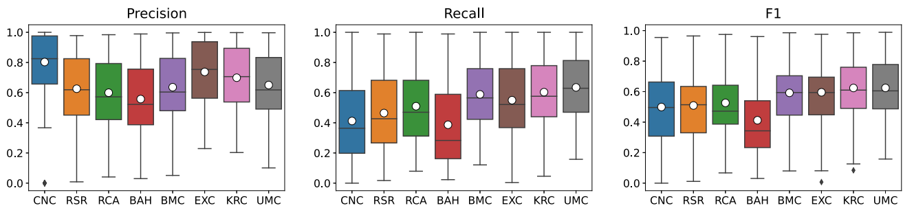
Fig. 4 Precision, recall and F1 of all algorithms over all similarity graphs
