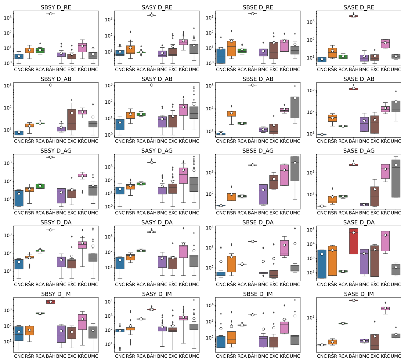
Fig. 7 The distribution of run-time (in ms) per algorithm and type of edge weights across the five smallest data sets. Every row corresponds to a different data set. Note the log-scale of the vertical
