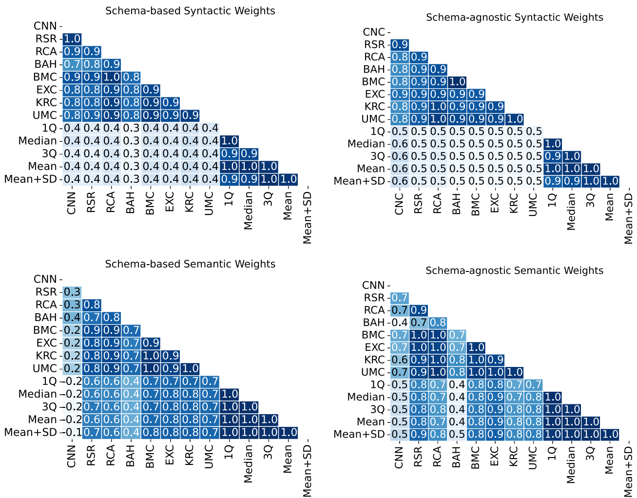
Fig. 14 Pearson correlation between the similarity thresholds of every algorithm as well as between the similarity thresholds and the descriptive statistics of the edge weights distribution
