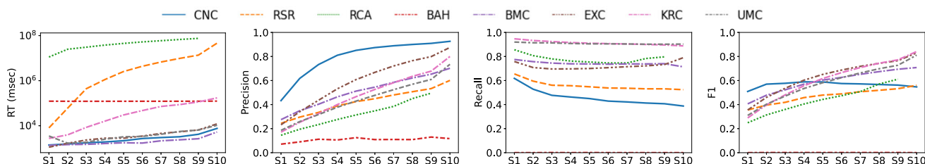
Fig. 11 Node scalability of all algorithms over the subsets in Table 4 with respect to run-time, precision, recall and F-Measure
