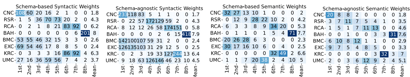
Fig. 9 Heatmaps summarizing the ranking positions per algorithm for each type of edge weights. Lower is better, i.e., the 1st ranking position corresponds to the fastest algorithm
