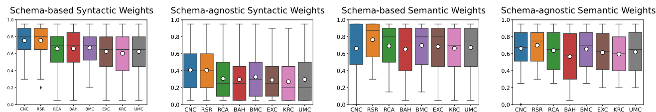
Fig. 13 The distribution of similarity thresholds per type of weights. White circles indicate the mean threshold in each case
