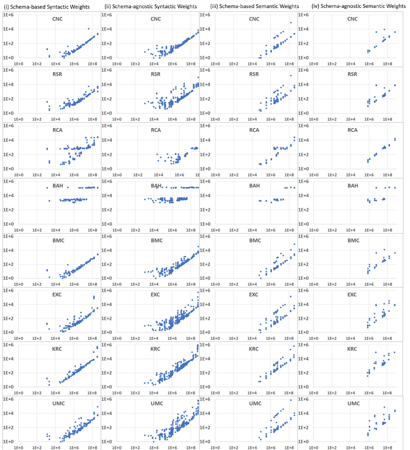
Fig. 10 Scalability analysis of all algorithms over all similarity graphs with (i) schema-based syntactic, (ii) schema-agnostic syntactic, (iii) schema-based semantic and (iv) schema-agnostic semantic edge
