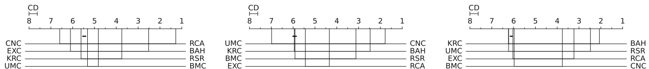
Fig. 5 Nemenyi diagrams based on precision, recall and F1 (from left to right)
