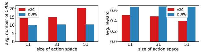
Fig. 4: Scalability over various sizes of action space
