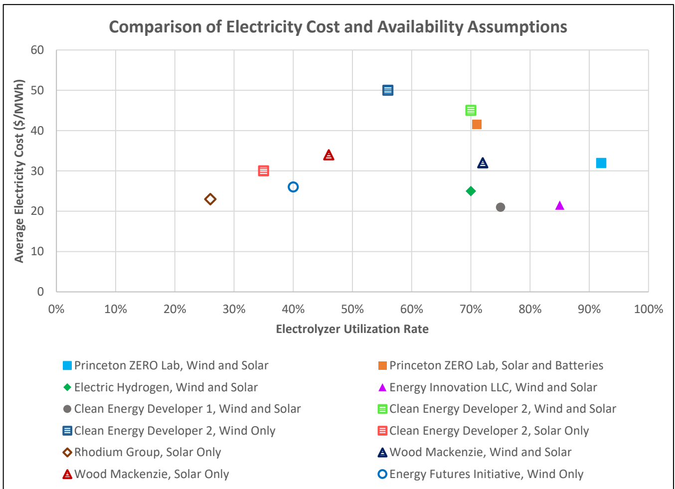
Figure 2: Average electricity cost and electrolyzer utilization rates from each study, including multiple cases where available. Filled markers indicate studies that allowed both oversizing of clean generating capacity and sales of excess clean generation. Patterned markers indicate studies that allowed oversizing but not excess sales. Unfilled markers indicate studies that assumed clean generating capacity to be equal to electrolyzer capacity.
