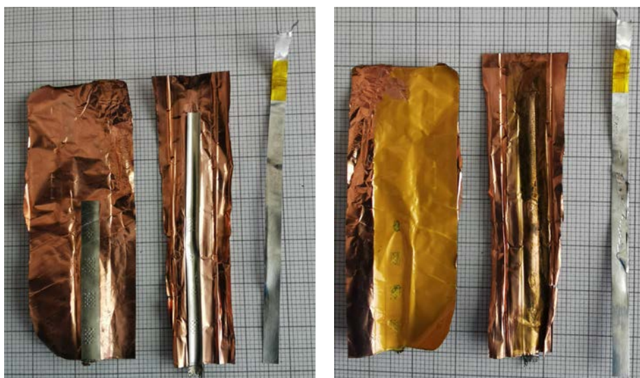
Figure 18. LG INR21700-M50LT
