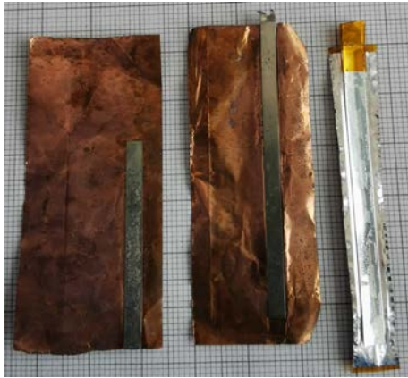
Figure 6. Sanyo UR18650RX
