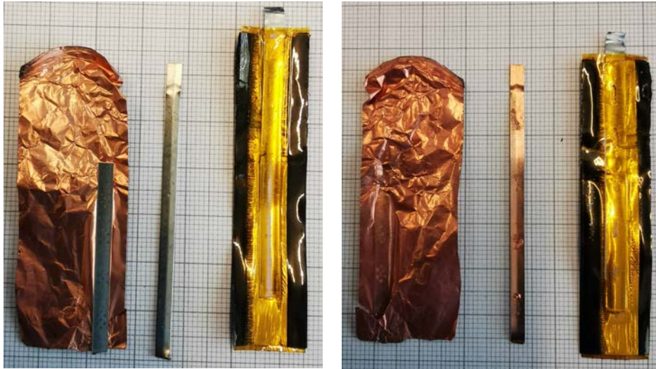
Figure 12. Panasonic NCR20700B
