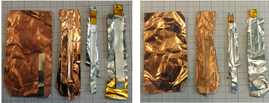
Figure 13. Sony / Murata US21700VTC6A
