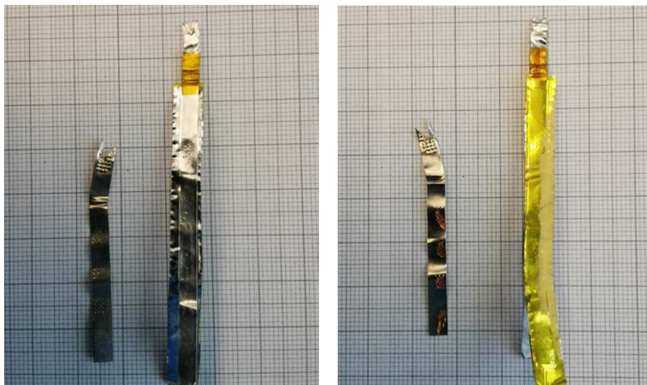
Figure 17. LG Chem INR21700-M50T
