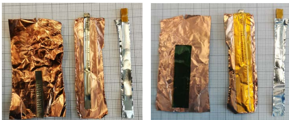
Figure 3. Samsung INR18650-25R
