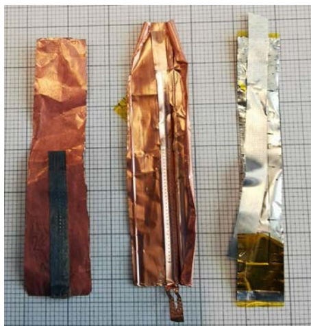
Figure 2. Sony / Murata US18650VTC6
