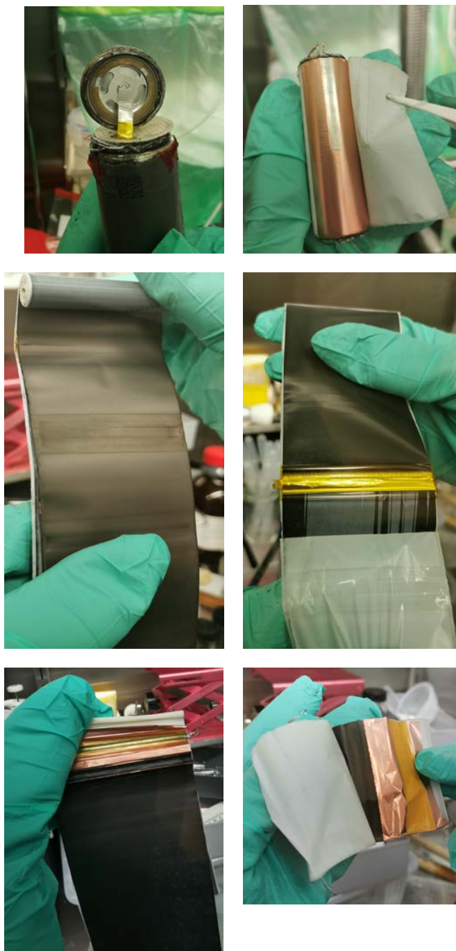
Figure 18. LG INR21700-M50LT
