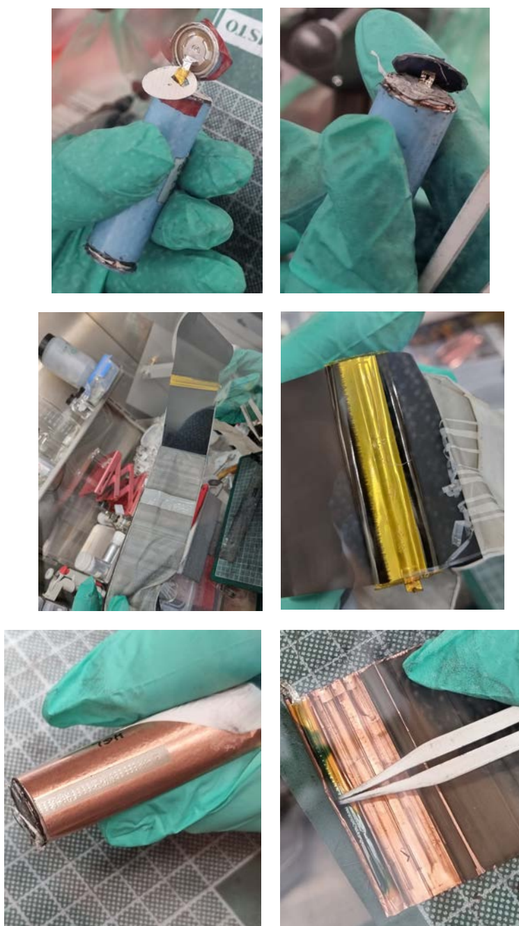
Figure 9. LG INR18650-HG2L
