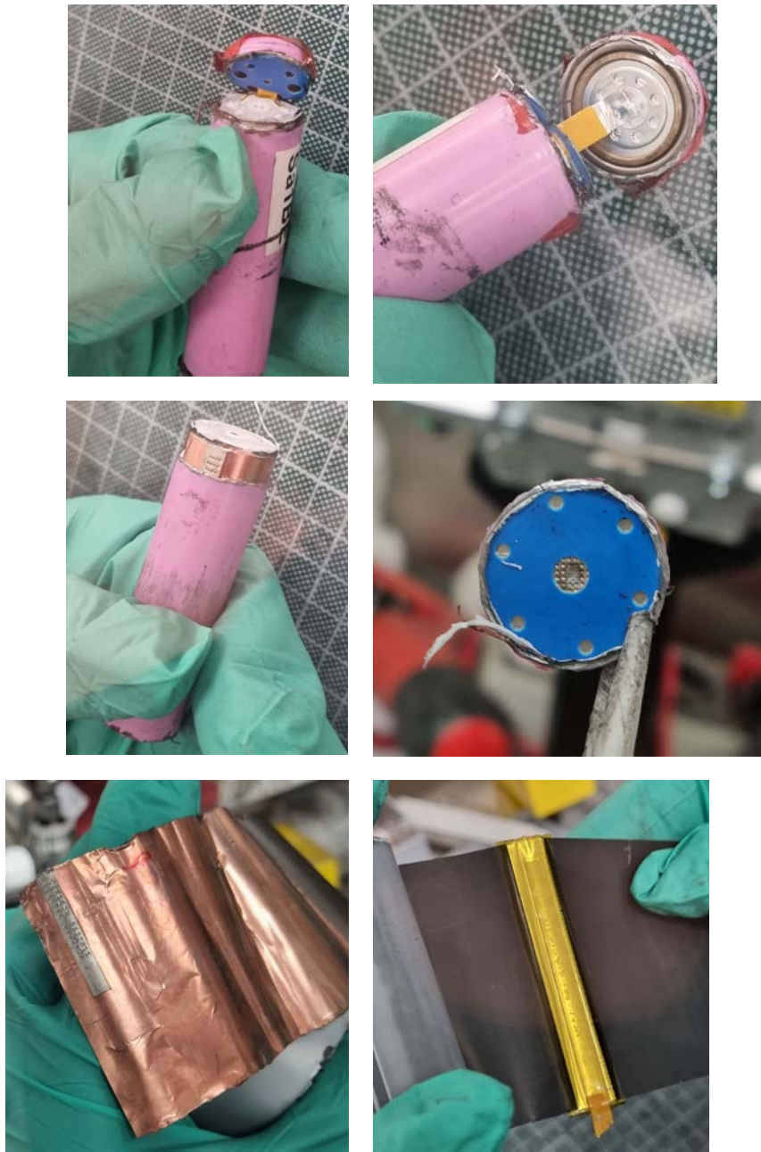
Figure 4. Samsung INR18650-35E
