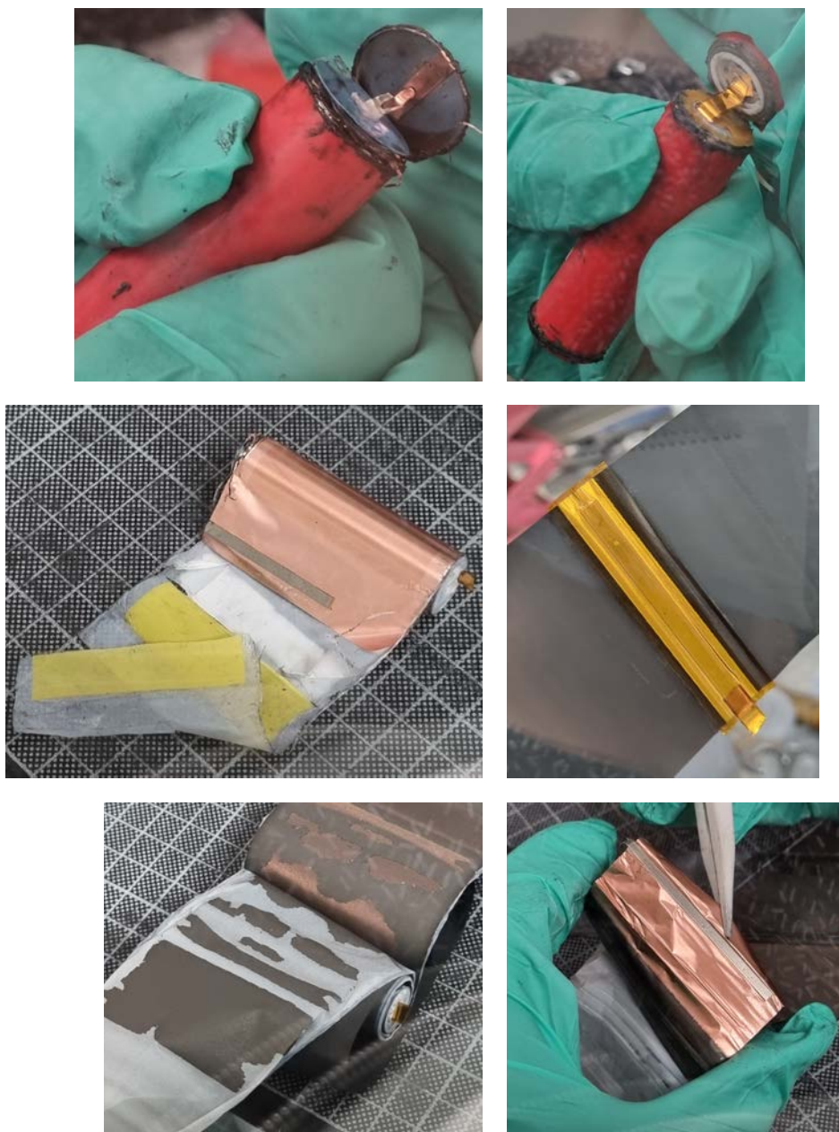
Figure 6. Sanyo UR18650RX
