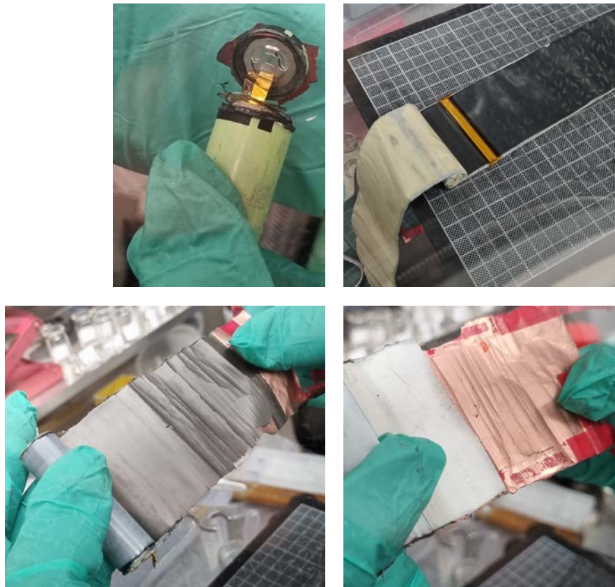
Figure 7. Panasonic NCR18650B
