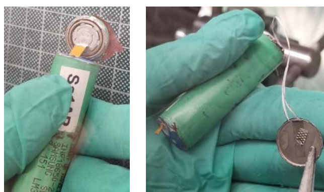
Figure 3. Samsung INR18650-25R
