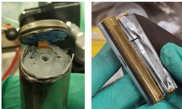
Figure 15. Samsung INR21700-33J
