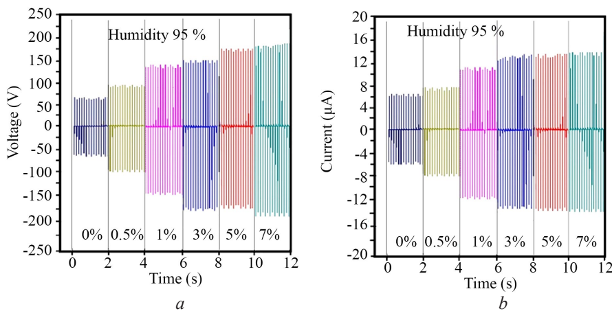
Fig. 11. Performance RDF-TENG at humidity 95 %:
