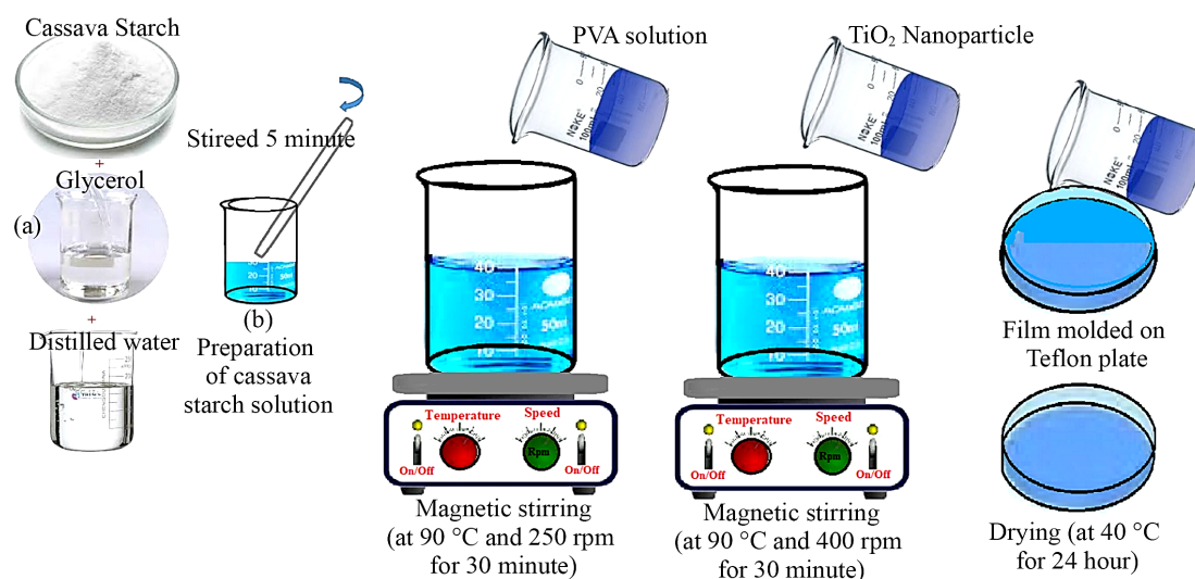
Fig. 1. Preparation of CS/PVA-TiO 2 nanocomposite films
