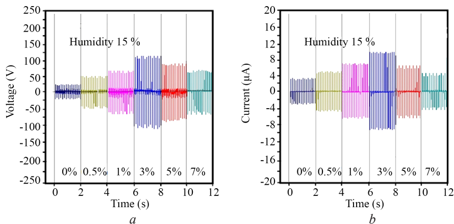
Fig. 10. Performance RDF-TENG at humidity 15 %:
