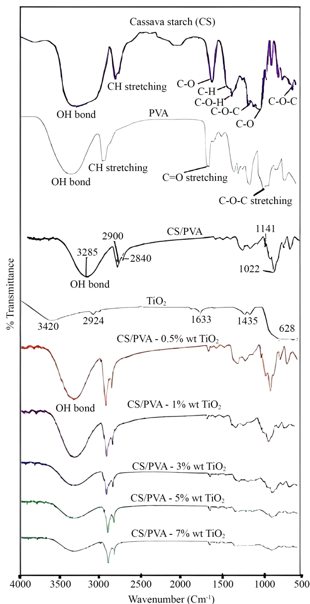
Fig. 3. Chemical formula analysis of cassava starch/PVA-TiO 2
