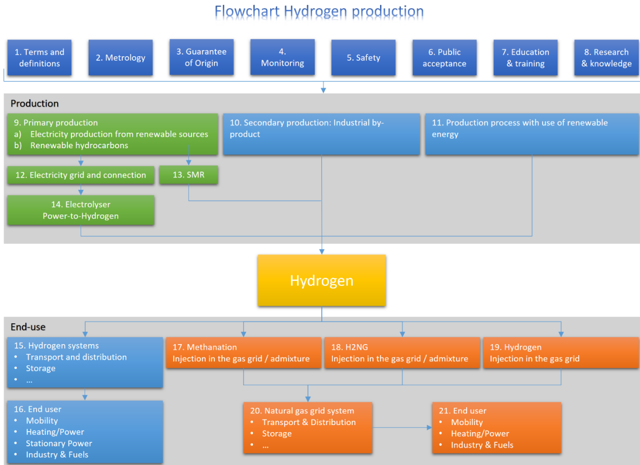
Figure 1: Flowchart of hydrogen production (own graphic) [19]
