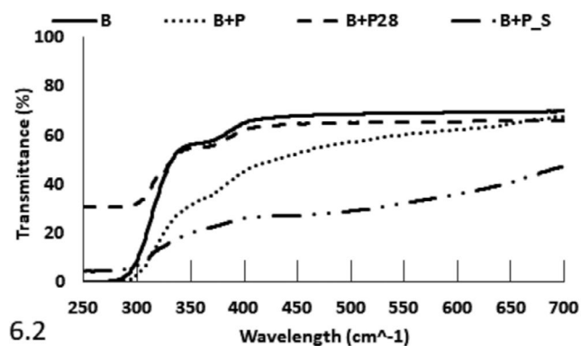
FIGURE 6 The reflectance spectra of hydroxyapatite and the transmittance spectra of SCNB through the use of UV-Vis spectroscopy. (6.1) Hydroxyapatite (H), functionalized hydroxyapatite (H+P), functionalized hydroxyapatite after the release test in water (H+P28) and functionalized hydroxyapatite after sterilization (H+P_S); (6.2) SCNB (B), functionalized SCNB (B+P), functionalized SCNB after the release test in water (B+P28), and functionalized SCNB after sterilization (B+P_S)
