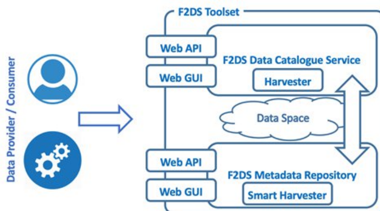
Figure 1. F2DS Overall Architecture
