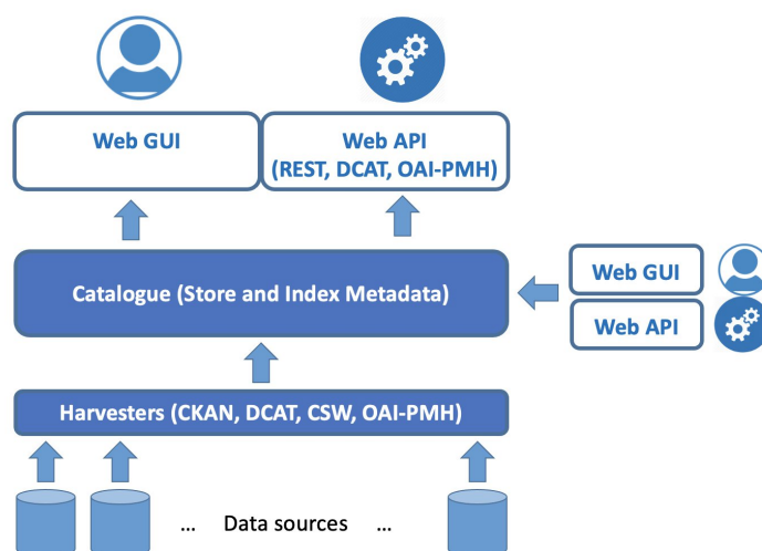
Figure 6. F2DS Catalogue Service Architecture
