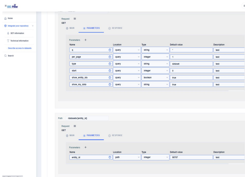
Figure 4. F2DS-Metadata Repository user interface: API description
