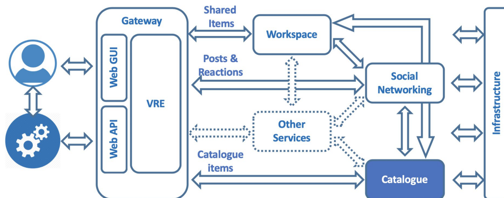
Figure 7. F2DS Data Catalogue integrated into a Virtual Research Environment
