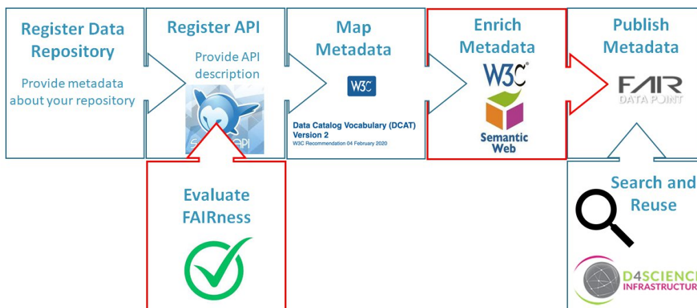
Figure 2. FFDS High-level Workflow
