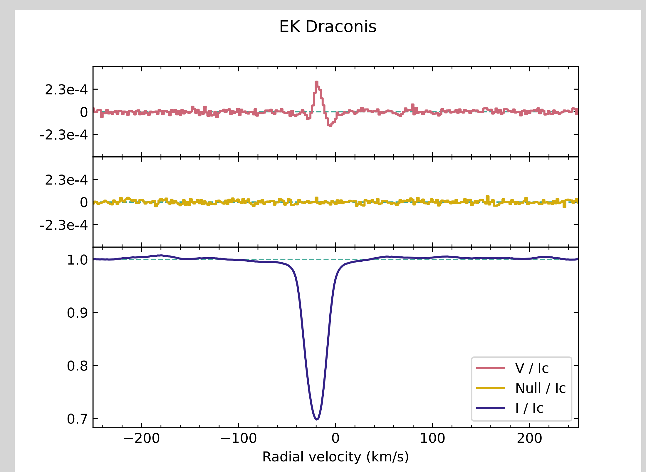
Cross-correlation profile for an observation of the active solar analogue EK Draconis. Top: circular polarization. Middle: « null » profile (control parameter
