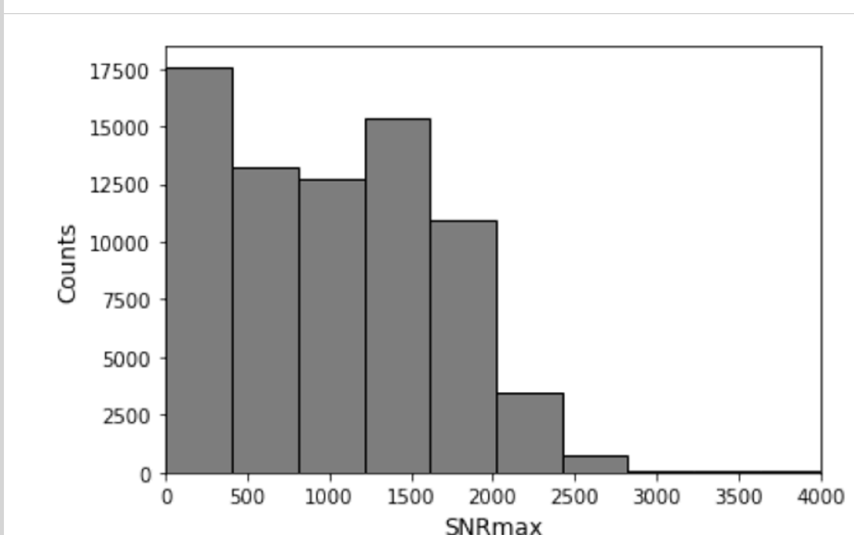
Top: distribution of visual magnitudes. Middle: distribution of stellar distances. Bottom: distribution of S/N (in the center of the spectral order where it is maximal). Note that close to 50% of observations benefit from a S/N greater than 1,000.
