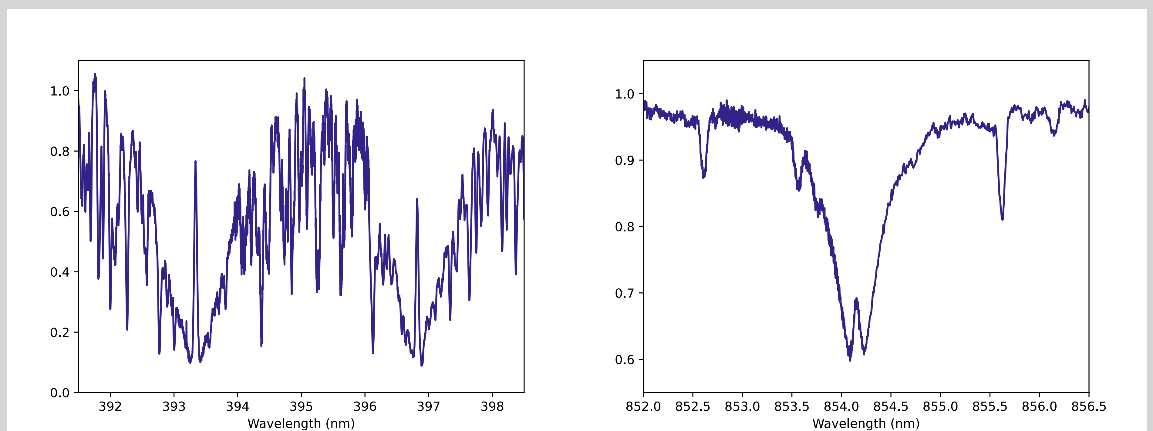
Zoom on selected spectral regions of an observation of the active Sun-like star EK Draconis. Left: the Call H&K doublet. Right: one line of the Call IR triplet.
