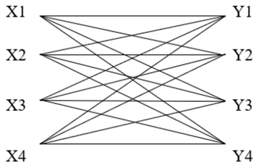
Figure 1. The graph of fuzzy relationships
