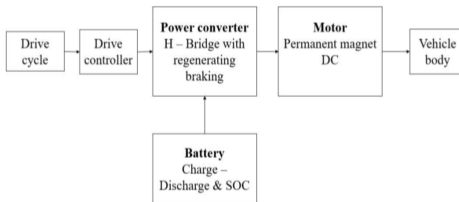
Figure 1: Block diagram of the proposed model
