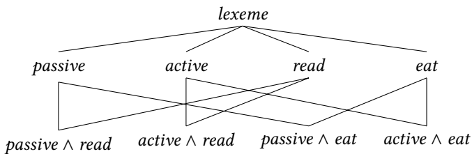
Figure 21.5: Inheritance Hierarchy for active and passive
