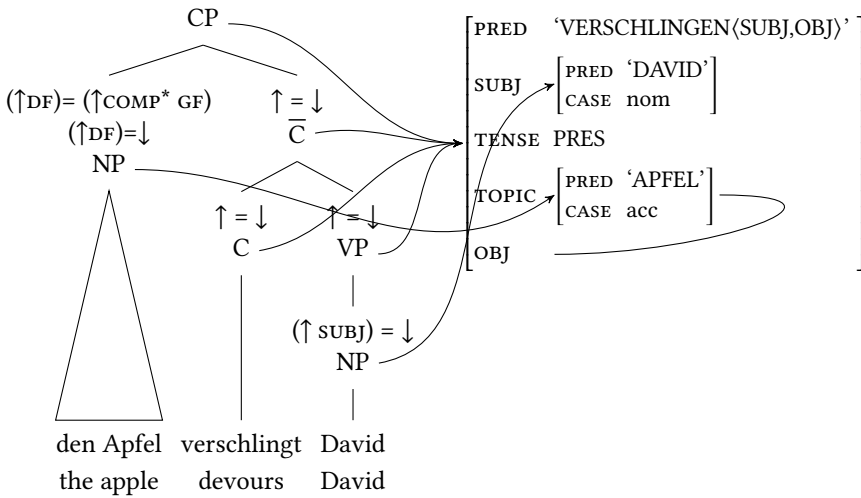
Figure 7.5: Analysis of verb second
