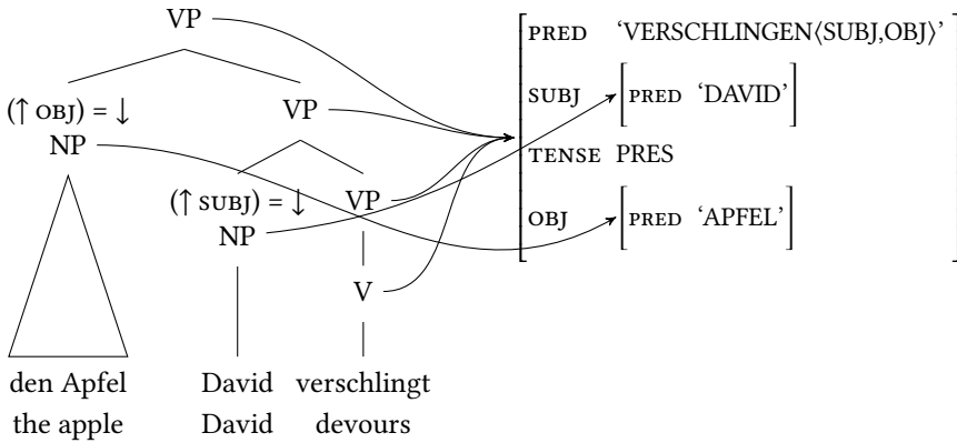
Figure 7.4: Analysis of OSV order following Berman (1996)
