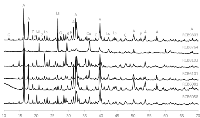
Figure 5. Diffractogram of artefact surface samples consisting of corrosion and soil minerals. A=atacamite; Cu=cuprite; Ls=lead sulphate; C=calcite; Q=quartz; G=gypsum; Z=zeolite; P=paratacamite.
