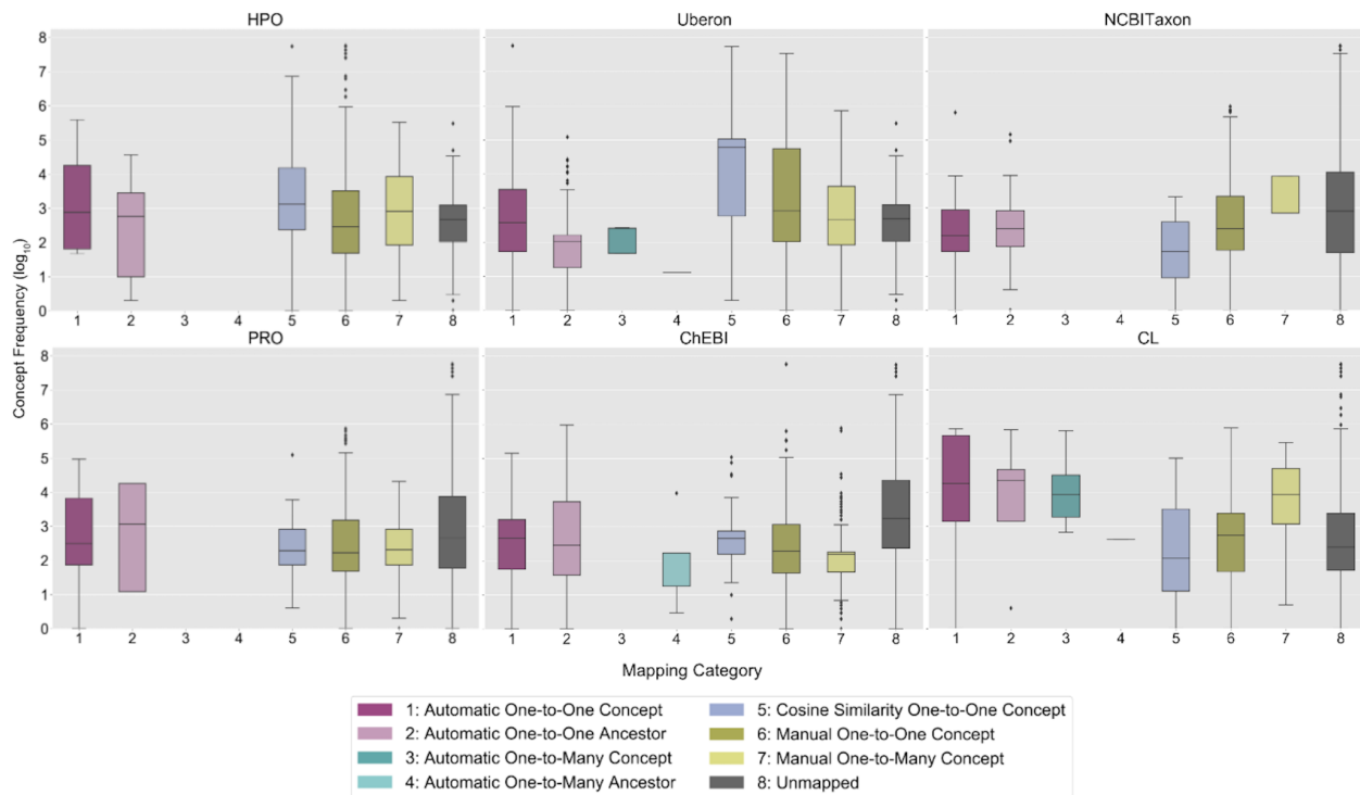
Figure 6: Measurement Concept Frequency of Use in Clinical Practice by Mapping Category and OBO Foundry Ontology.
