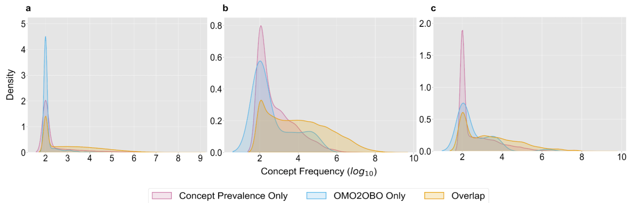
Figure 7: OMOP2OBO - Concept Prevalence Coverage.
