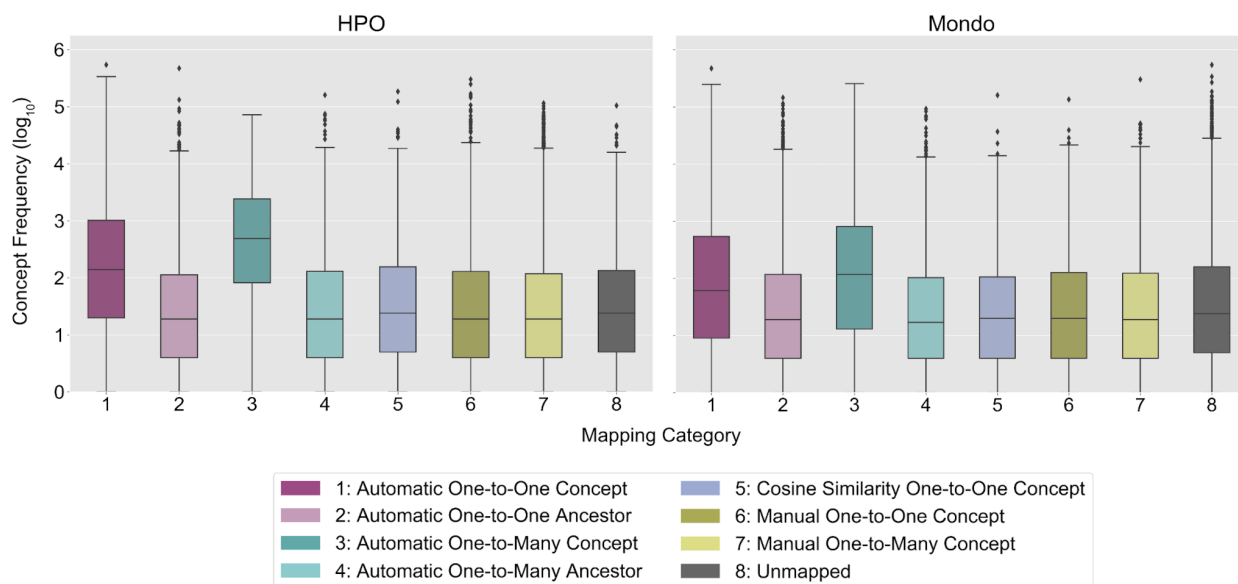
Figure 4: Condition Concept Frequency of Use in Clinical Practice by Mapping Category and OBO Foundry Ontology.
