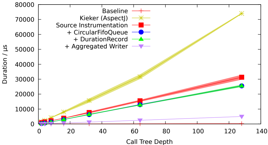
Kieker Overhead Reductions Measurement Durations
