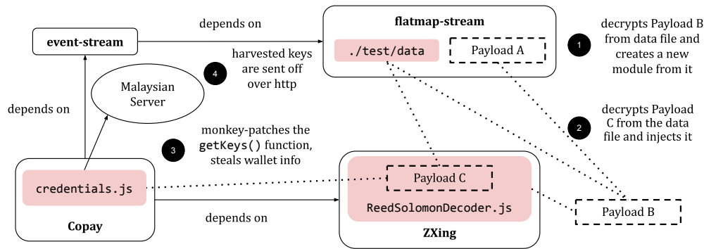
Fig. 2: An overview of the interactions between files and modules.
