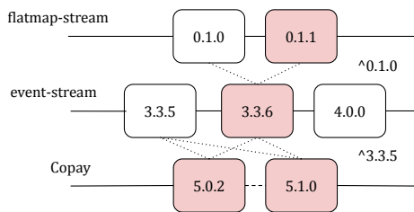
Fig. 1: Package dependency graph along with relevant versions. Highlighted in red are versions shipped with the malicious code.
