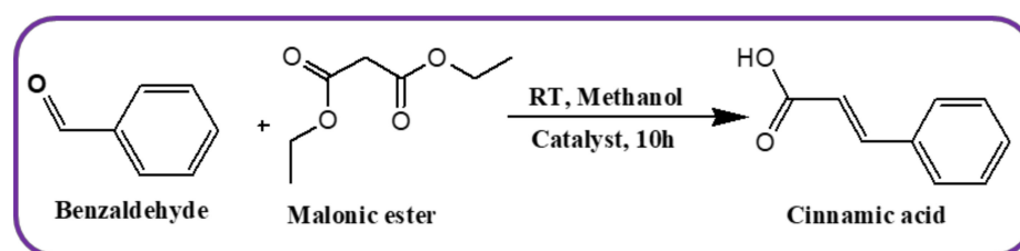
Scheme 2. Schematic presentation of Knoevenagel condensation reaction.
