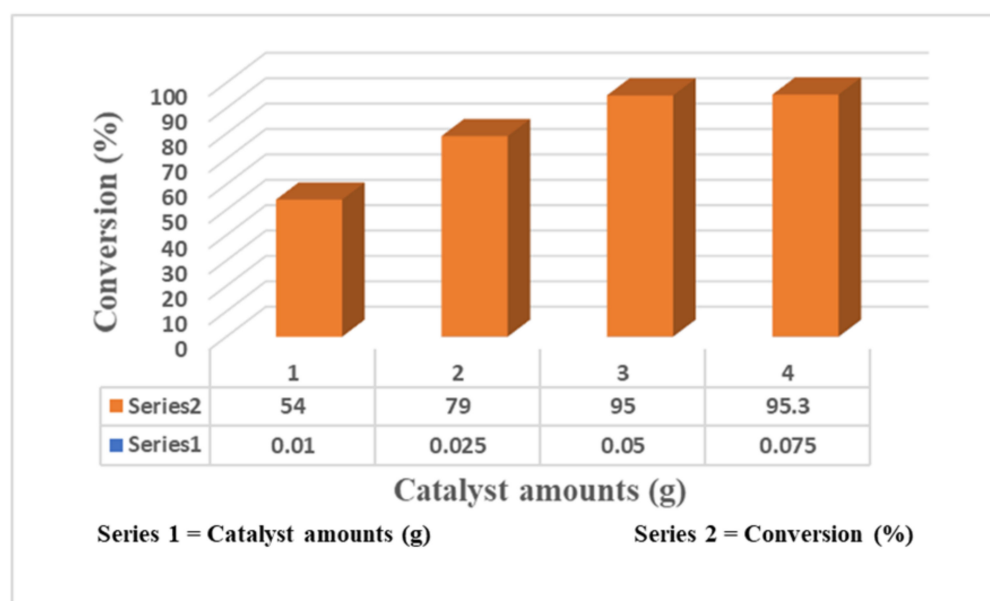
Figure 2. Variation of catalyst amounts of 12.8-A-MCM-41-S catalyst over Knoevenagel condensation reaction.
