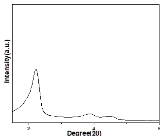
Figure 4. XRD spectrum of the reused catalyst after the fourth cycle.
