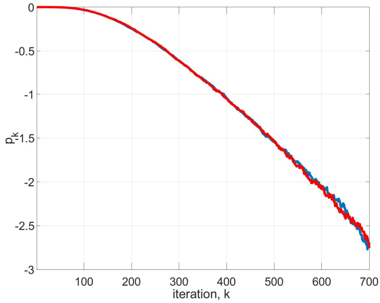
Figure 1: Monte Carlo estimate of P(\|X_k - x^*\| > \delta) along iterations k = 1, 2, \dots for SGD with Gaussian (blue line) and Laplacian (red line) gradient noise with equal per-entry variance \sigma^2 = 0.04 . Top Figure: \delta = 0.3 ; Bottom Figure: \delta = 0.03 .
